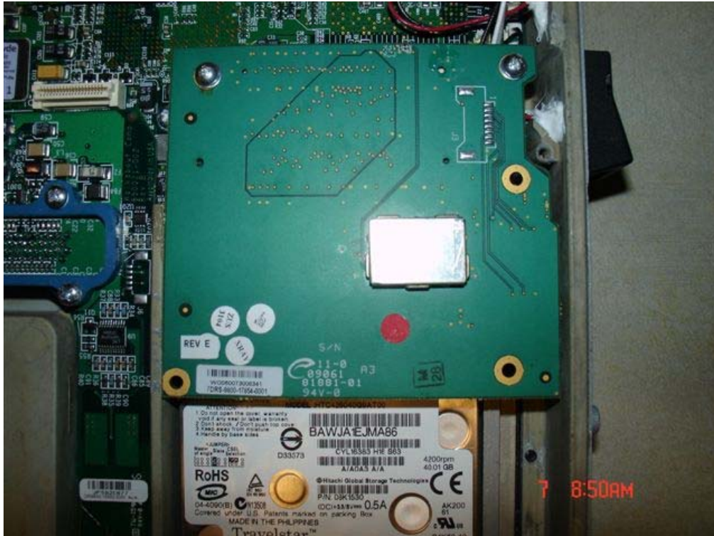
WIFI_BT SHIELDED
