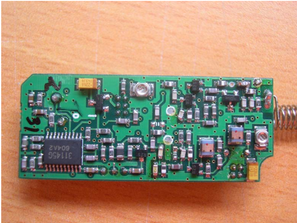
<Photograph 2: Front View> RF Board
