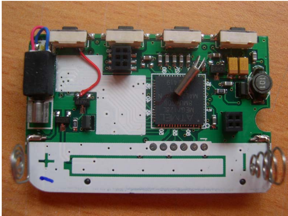
<Photograph 5: Rear View> Main Board
