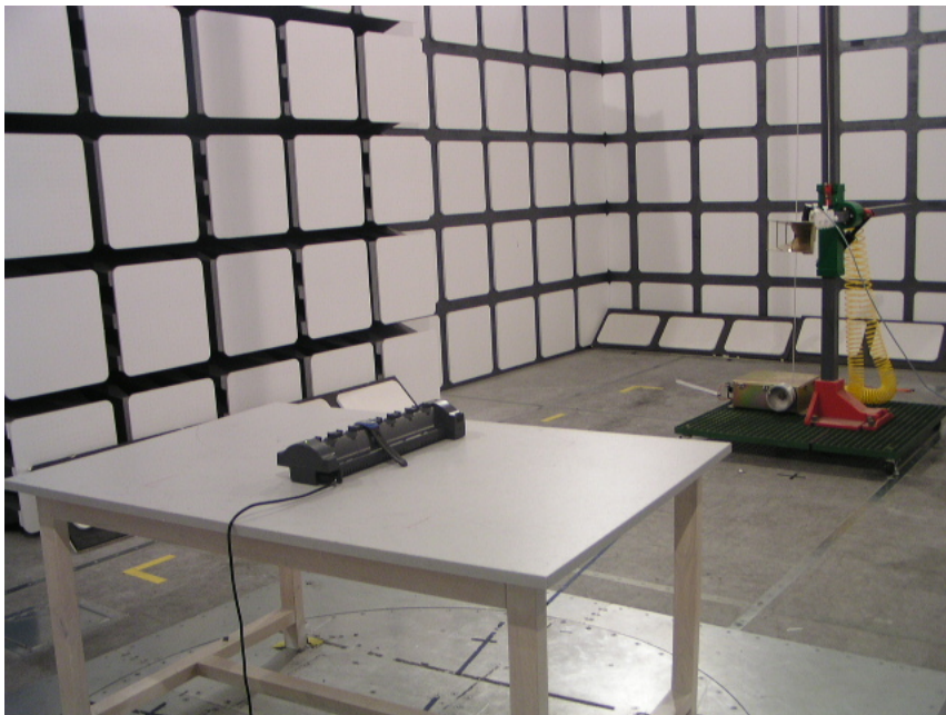
Charging Mode: Radiated Emission – Rear View (Above 1GHz)
