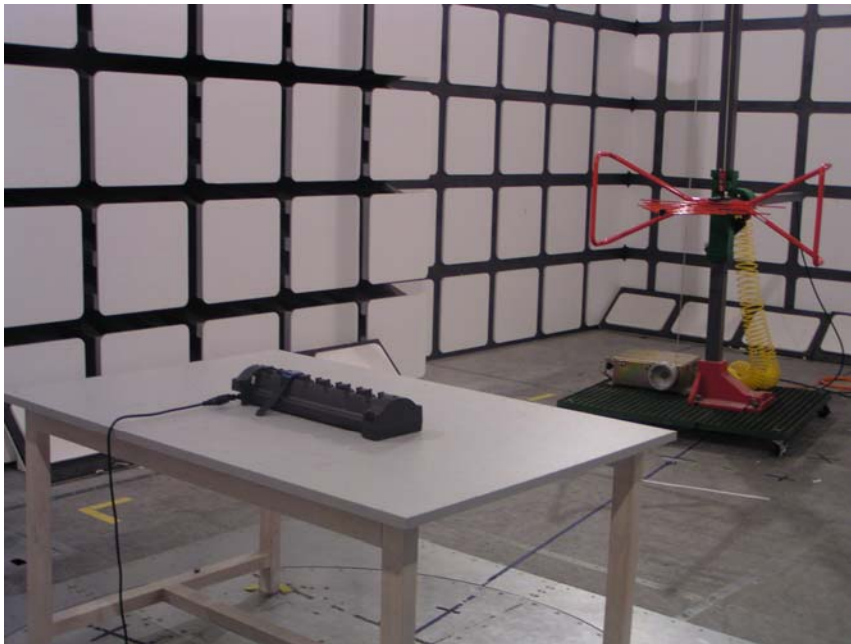
Charging Mode: Radiated Emission - Rear View (up to 1GHz)
