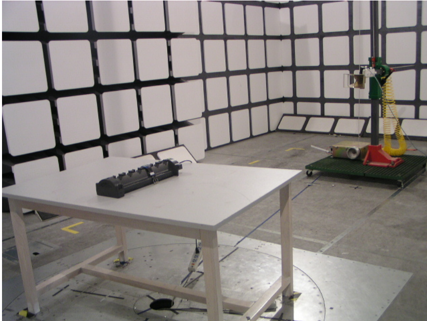
Charging Mode: Radiated Emission – Front View (Above 1GHz)
