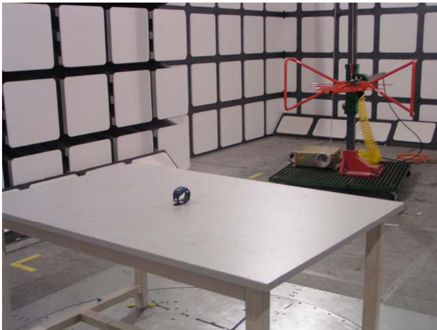
Transmitting Mode: Radiated Emission - Rear View (up to 1GHz)
