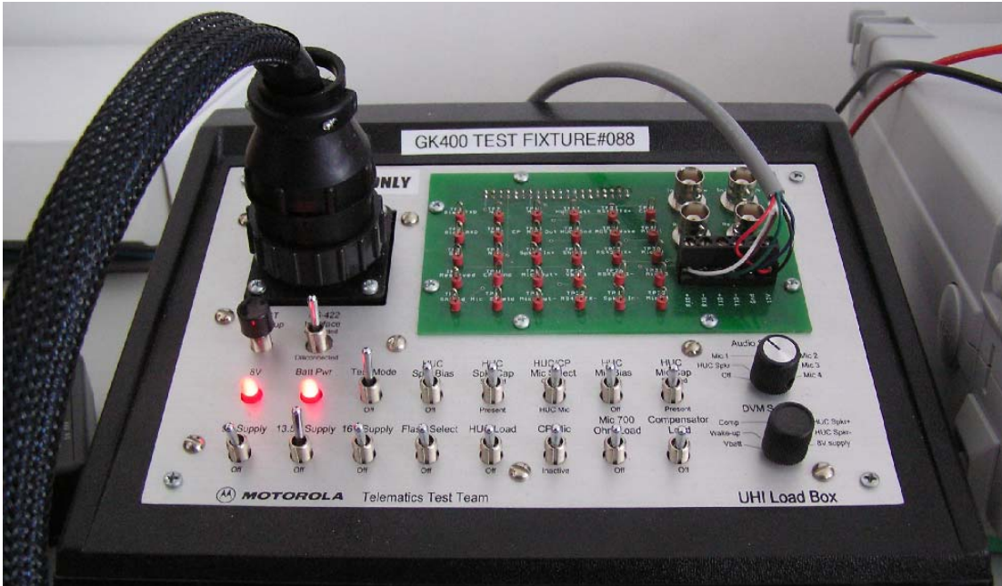
Photo 5: Test fixture GK400 #088
