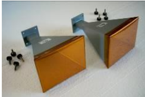
Fig. 3 – Example of antennas with screw
