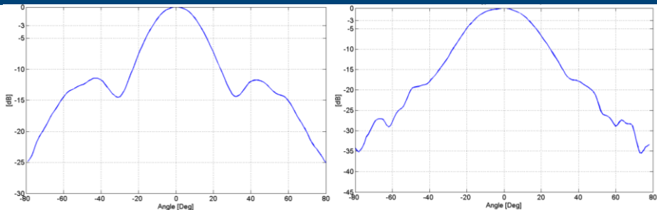
Figure B – Elevation and Azimuth ANT2 Pattern
