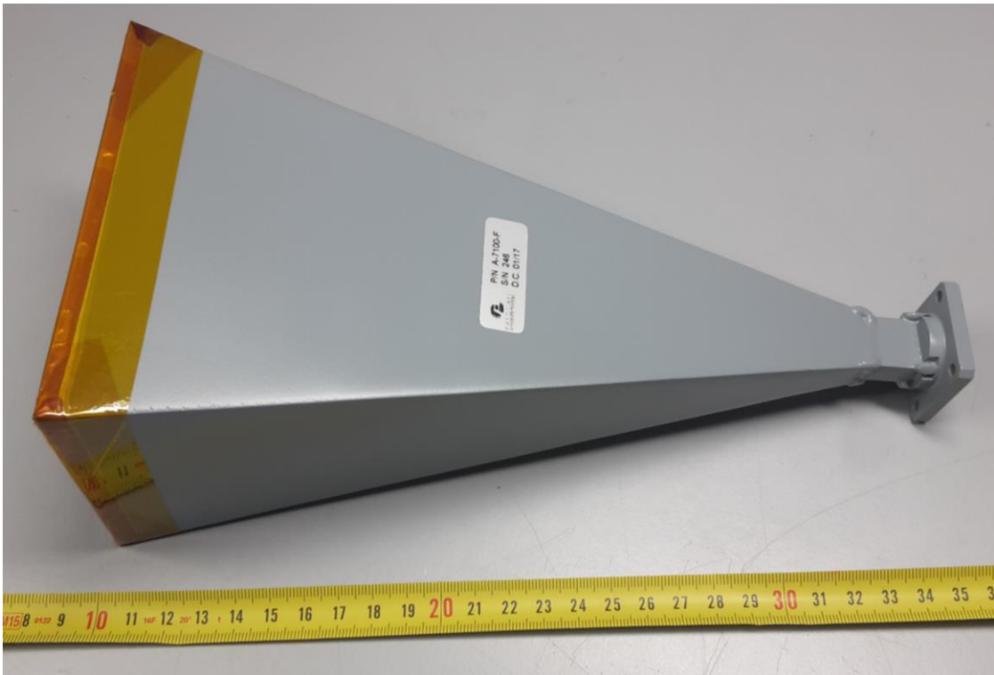
Antenna 4 (IBIS-ANT4-H11V10) – Bottom View
