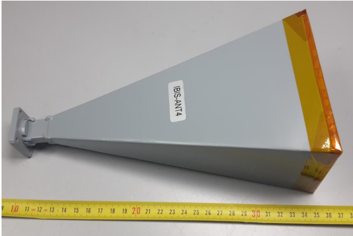
Antenna 4 (IBIS-ANT4-H11V10) – Top View
