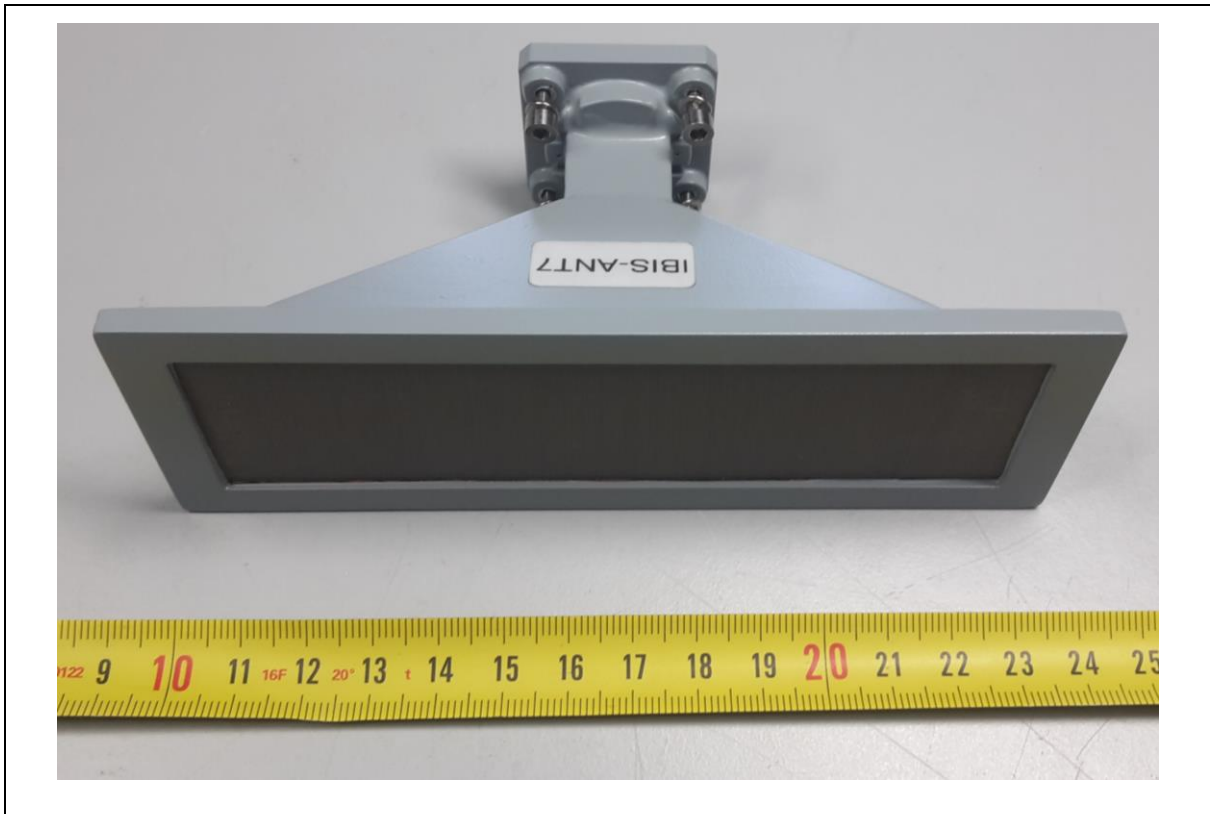
Antenna 7 (IBIS-ANT7-H50V31) – Front View
