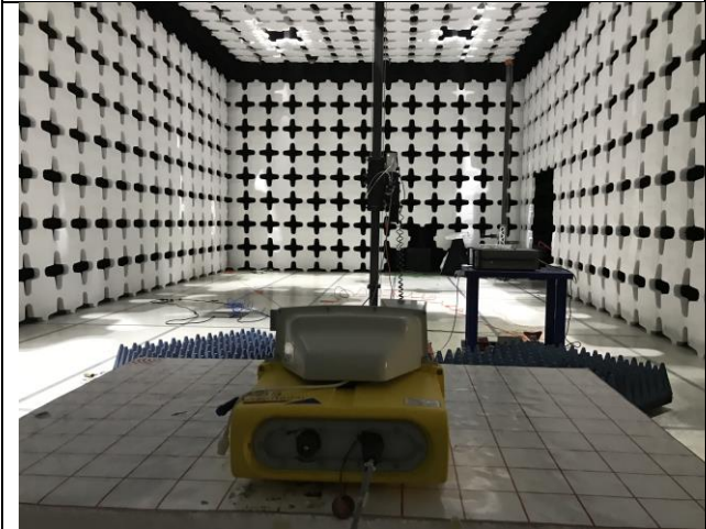
Radiated Emissions (18-40GHz) – Front View
