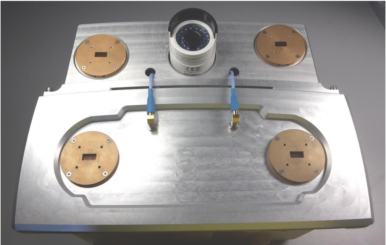
Fig. 3 – IBIS Sensor with optional MIMO Kit - Front view
