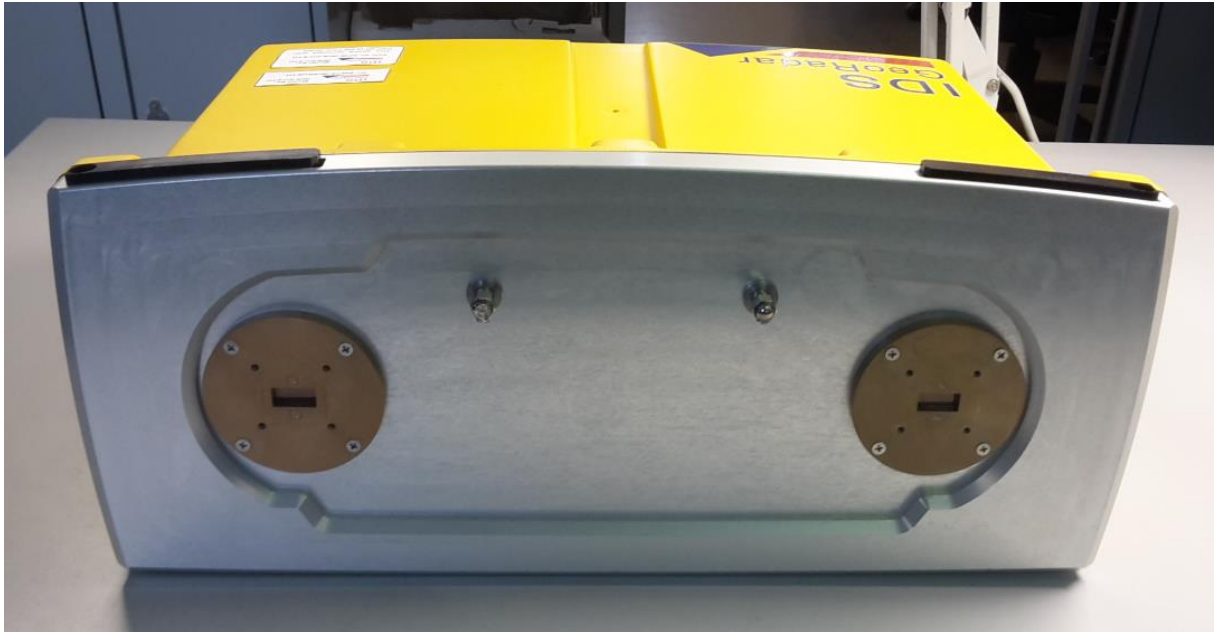
Fig. 1 – IBIS Sensor - Front view
