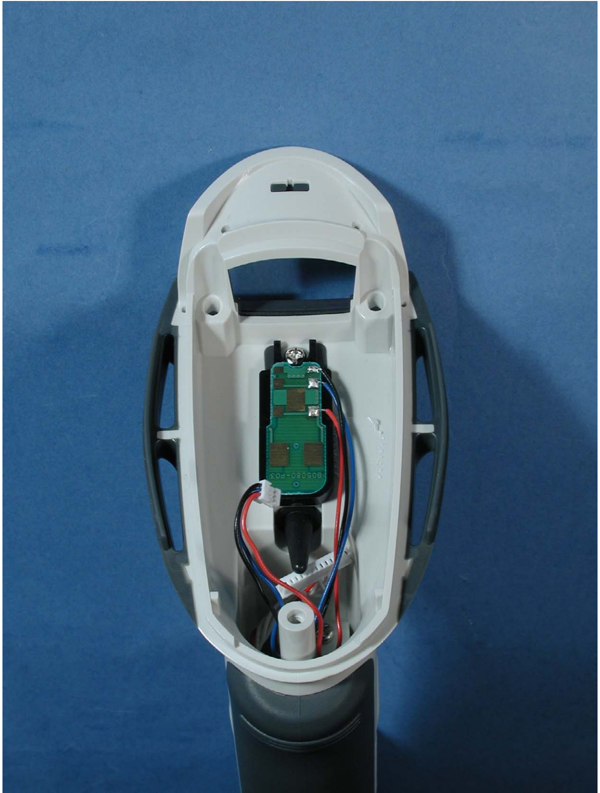
Photograph 2: - Scanner OPR-3101, inside view 2
