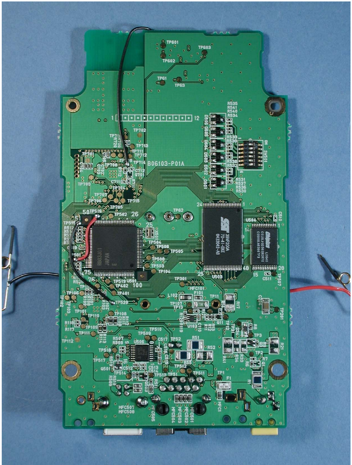
Photograph 11: - Cradle CRD-3101 PCB, rear view
