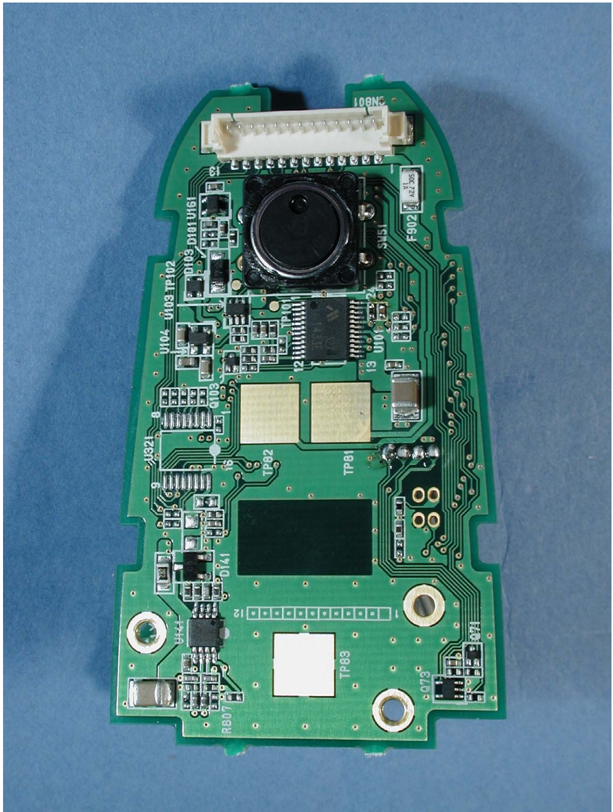
Photograph 3: - Scanner OPR-3101, main PCB, top view
