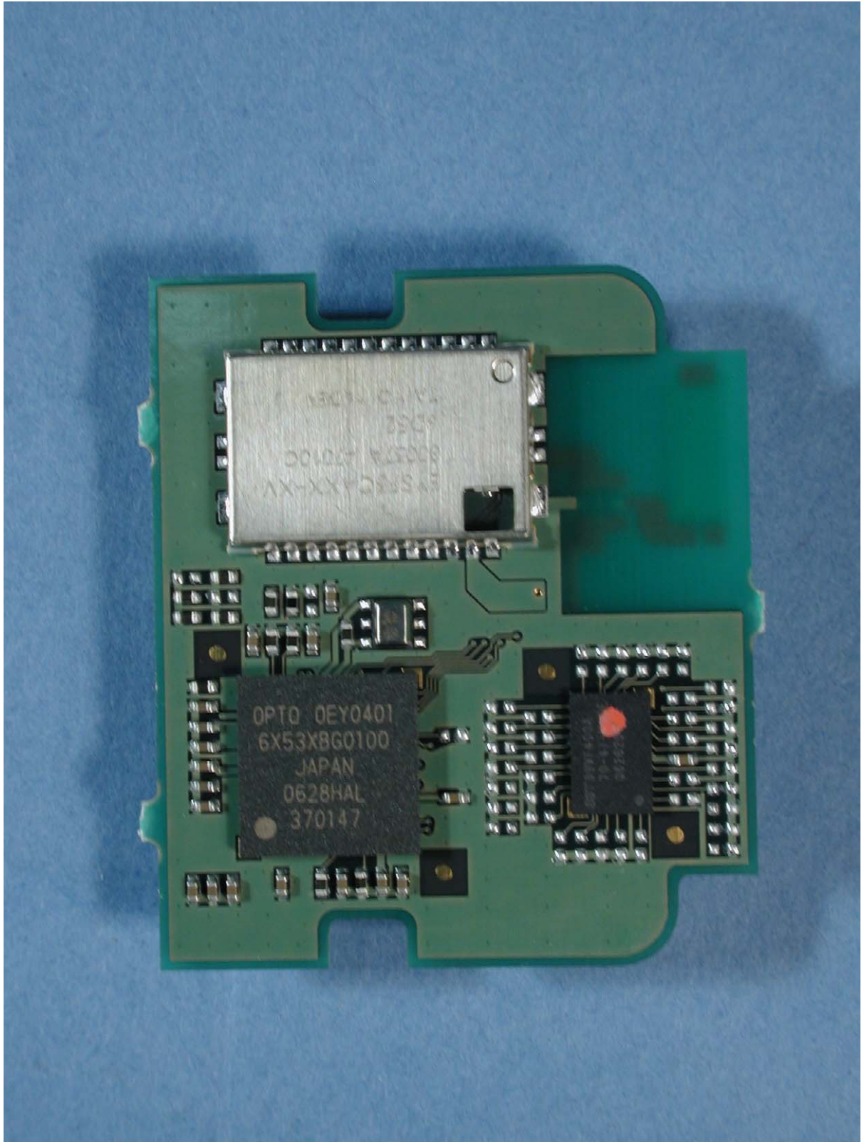
Photograph 6: - Scanner OPR-3101, decode PCB, rear view
