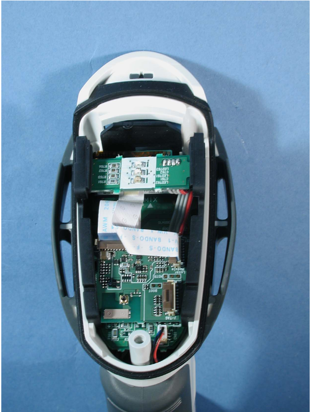
Photograph 1: - Scanner OPR-3101, inside view 1
