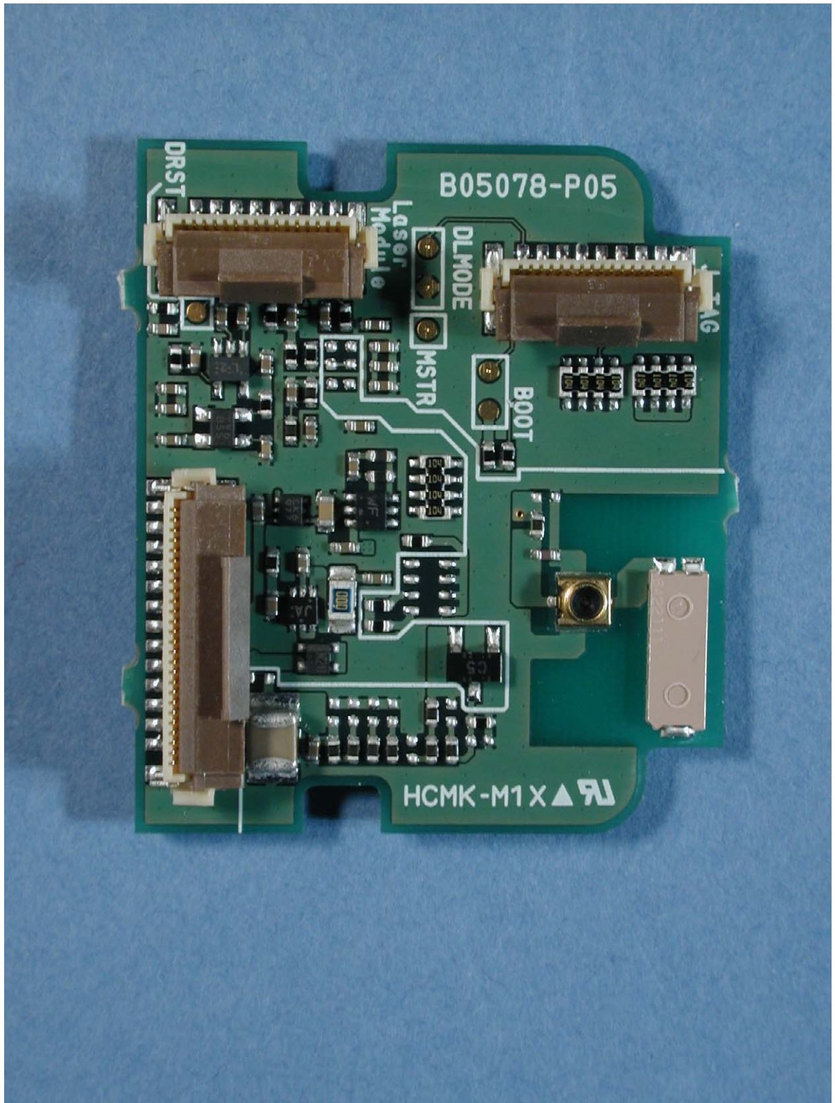
Photograph 5: - Scanner OPR-3101, decode PCB, top view
