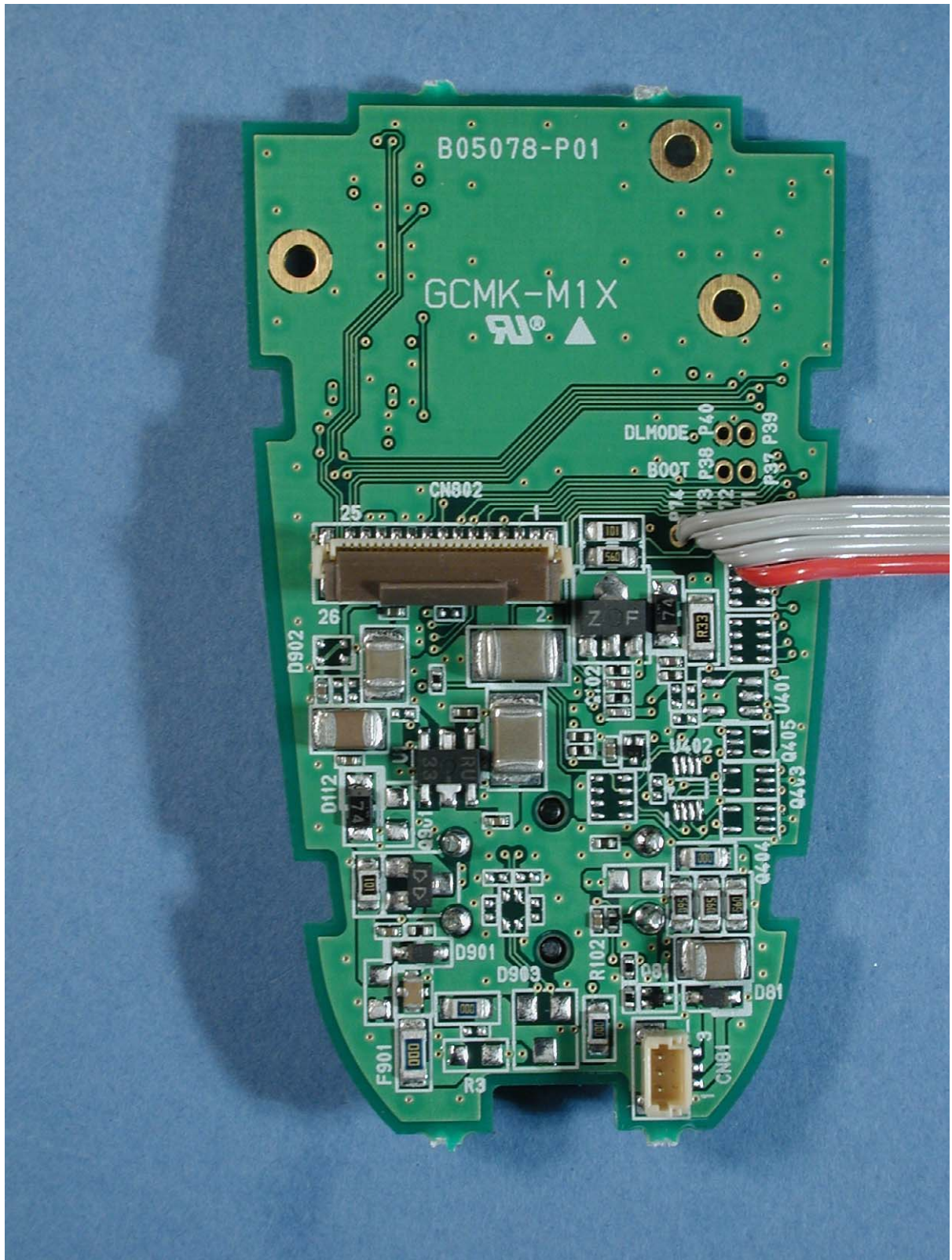
Photograph 4: - Scanner OPR-3101, main PCB, rear view
