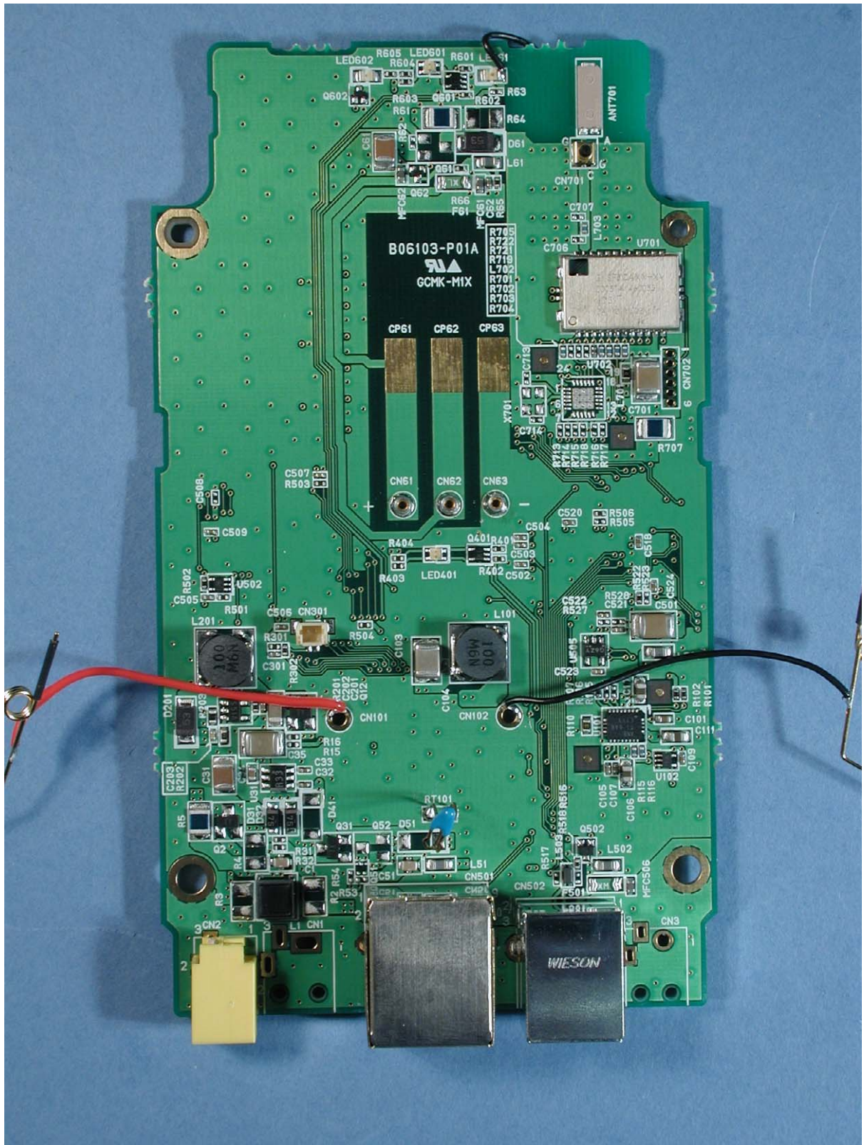
Photograph 10: - Cradle CRD-3101 PCB, top view
