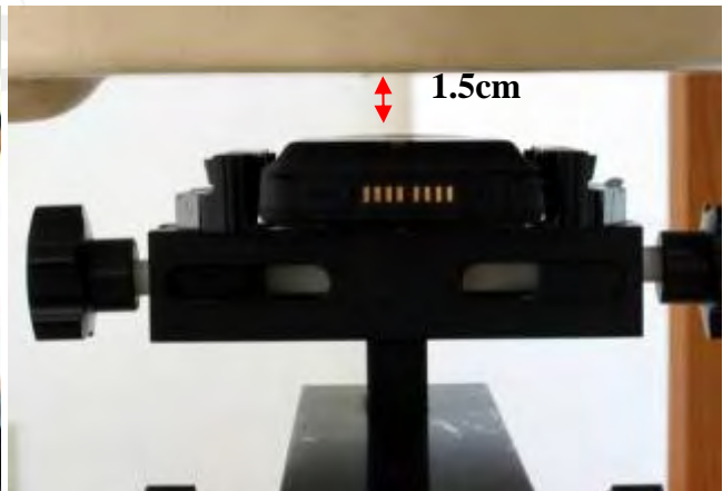
Fig.8 Body worn- EUT back to flat phantom and distance between flat phantom and mobile phone is 1.5 cm
