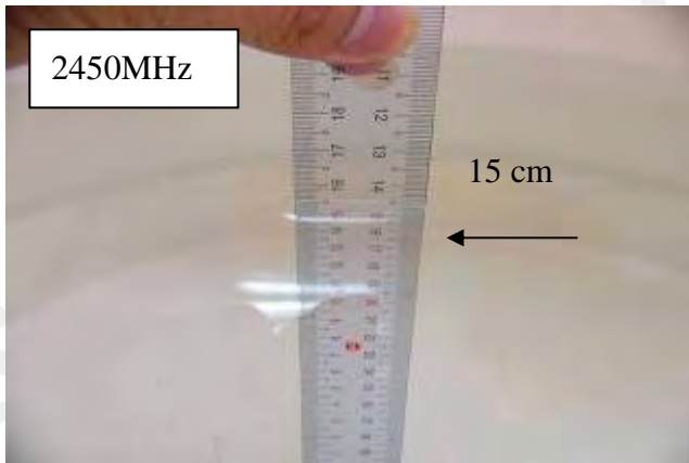
Fig.2.5 Photograph of the Tissue Simulant Fluid liquid depth 15cm for Flat (Body)
