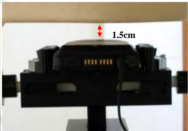
Fig.9 Body worn- EUT back to flat phantom and distance between flat phantom and mobile phone is 1.5 cm
