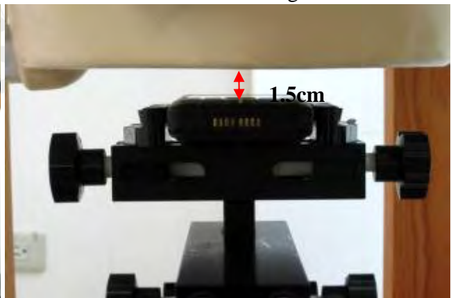
Fig.7 Body worn- EUT front to flat phantom and distance between flat phantom and mobile phone is 1.5 cm
