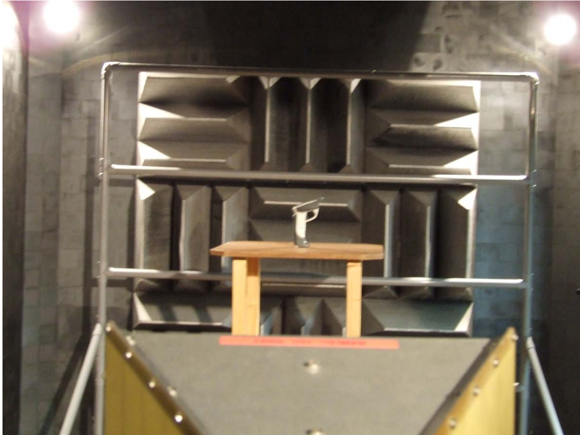
Photograph 2: Test setup Radiated Emissions (> 1 GHz) Scanner OPR-3101
