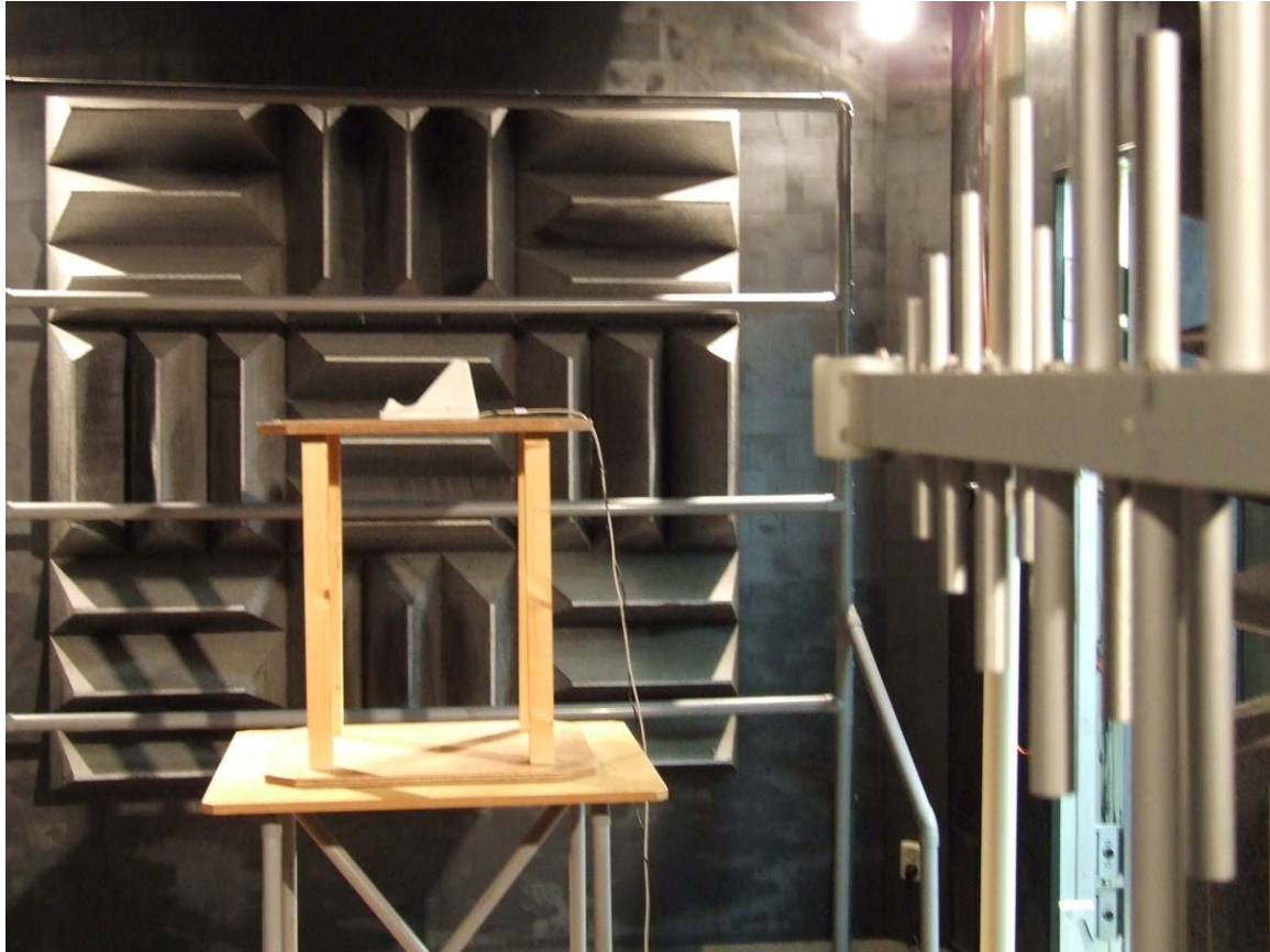
Photograph 4: Test setup Radiated Emissions (< 1 GHz) Cradle CRD-3101
