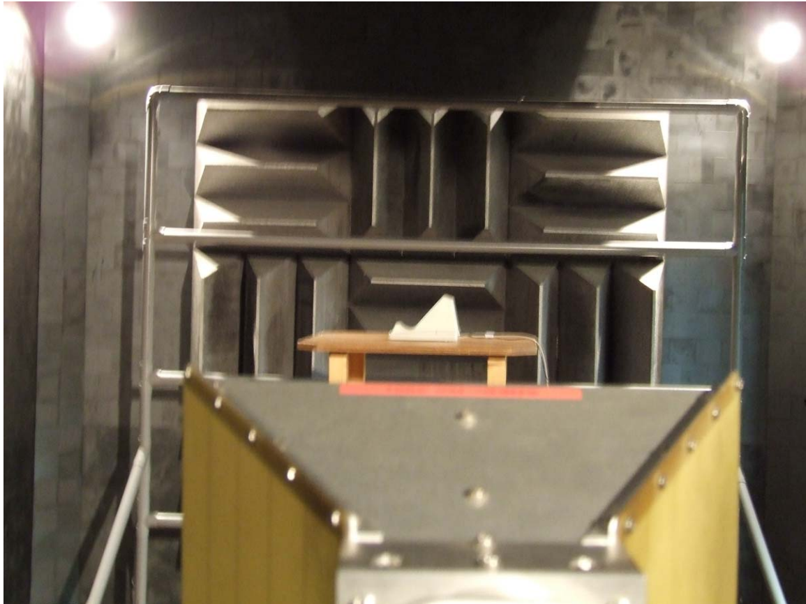
Photograph 5: Test setup Radiated Emissions (> 1 GHz) Cradle CRD-3101
