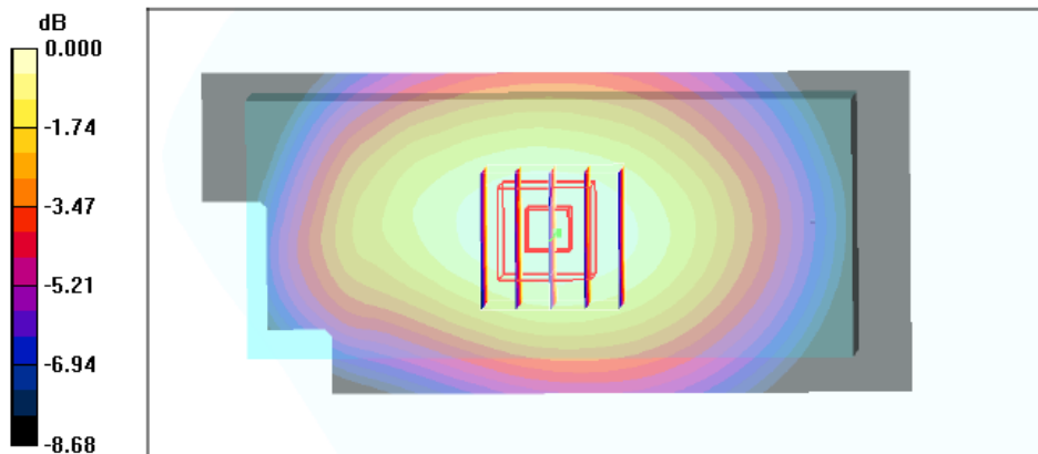
0 dB = 0.181mW/g
