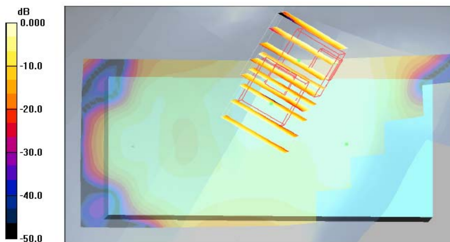
0 dB = 0.036mW/g
