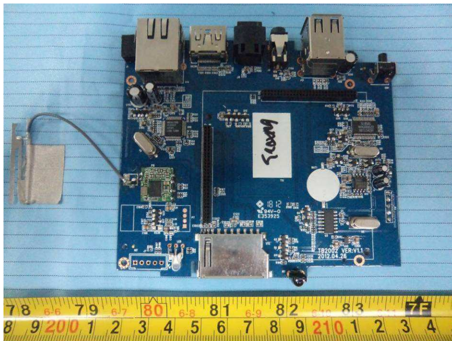
EUT –TB2002 V1.1 Board Top View
