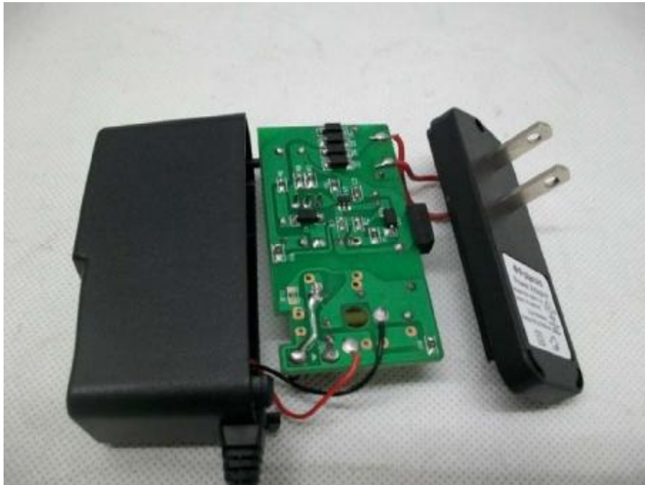
INTERNAL PHOTO OF POWER SUPPLY - 1
