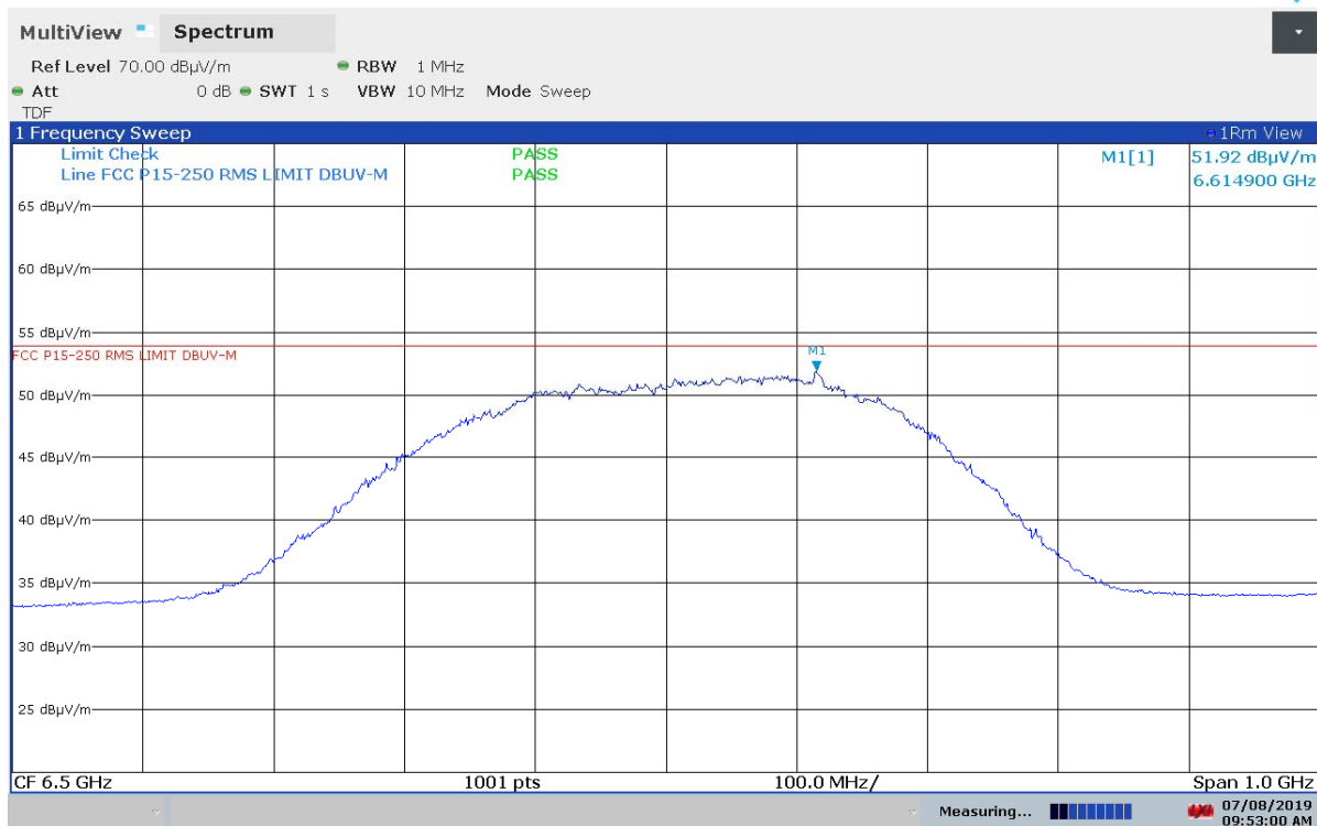
293-19 iRobot Wideband Confinement Beacon
