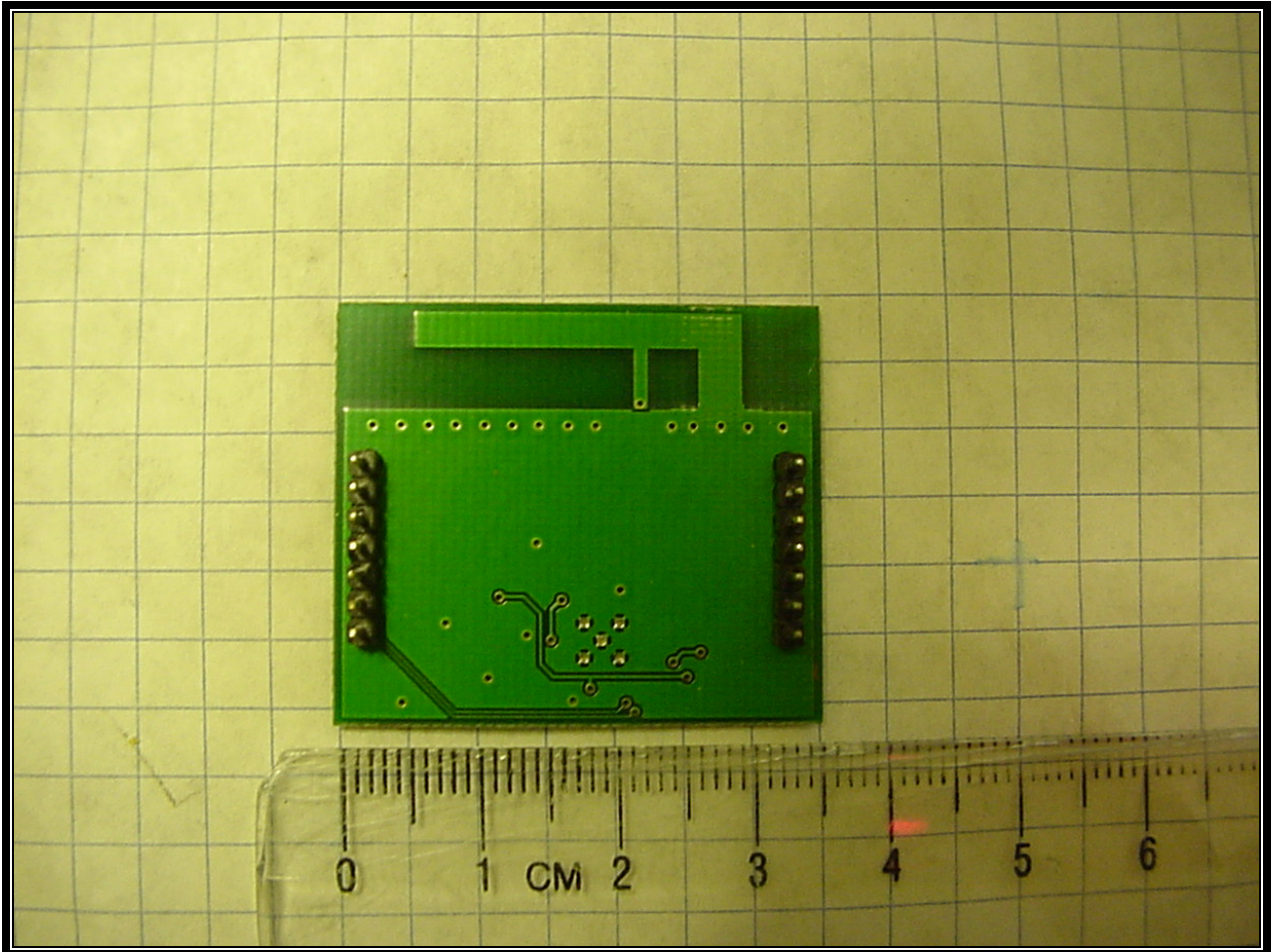
Photograph 5: Bottom View
