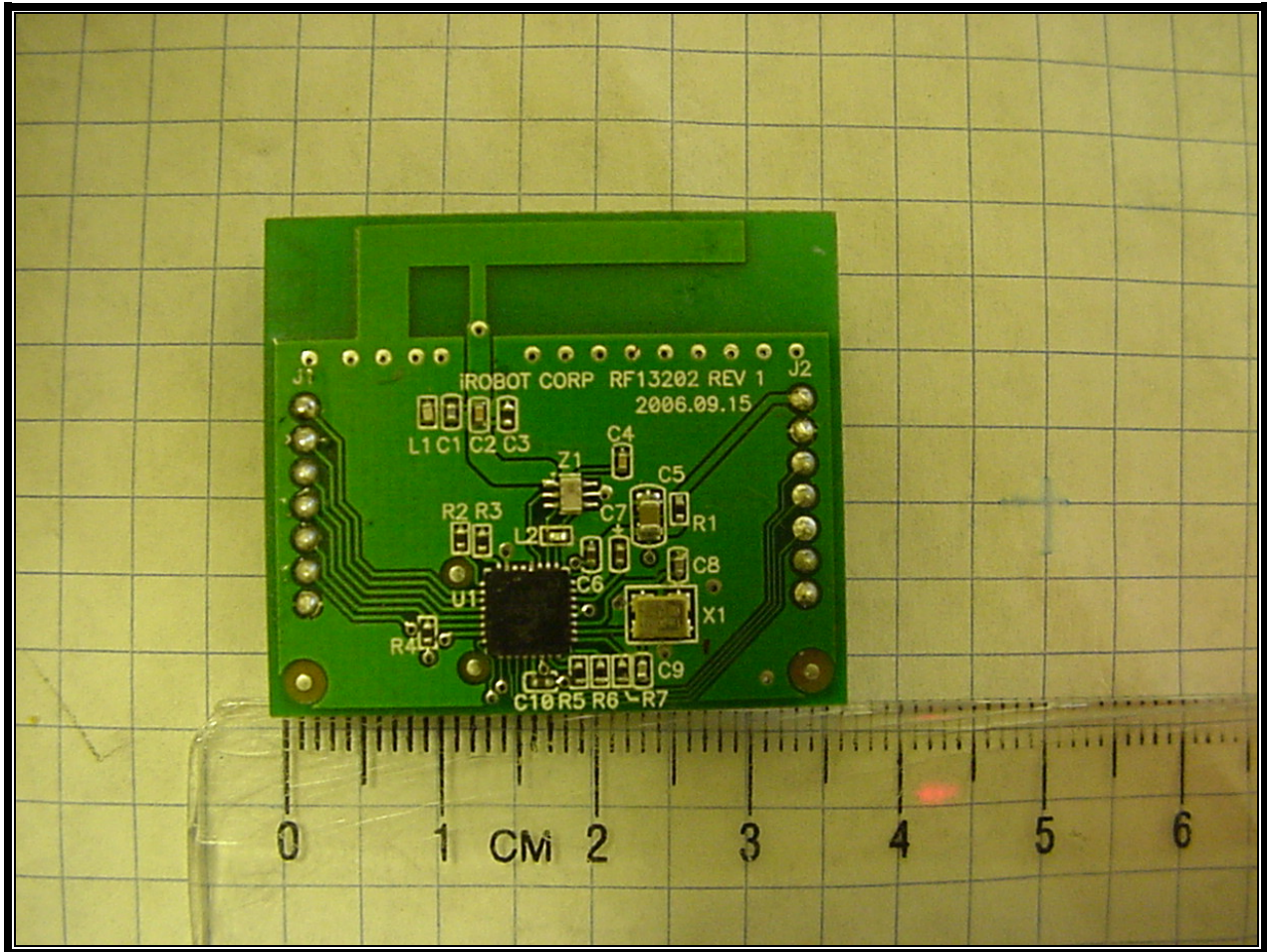
Photograph 4: Top View
