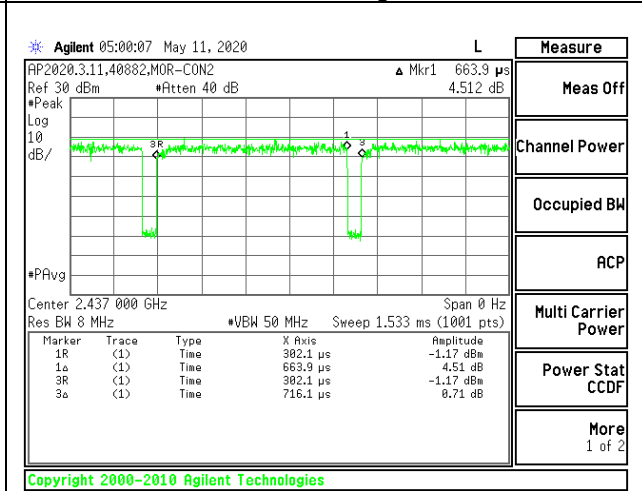
DUTY CYCLE 802.11n HT40 SDM MODE
