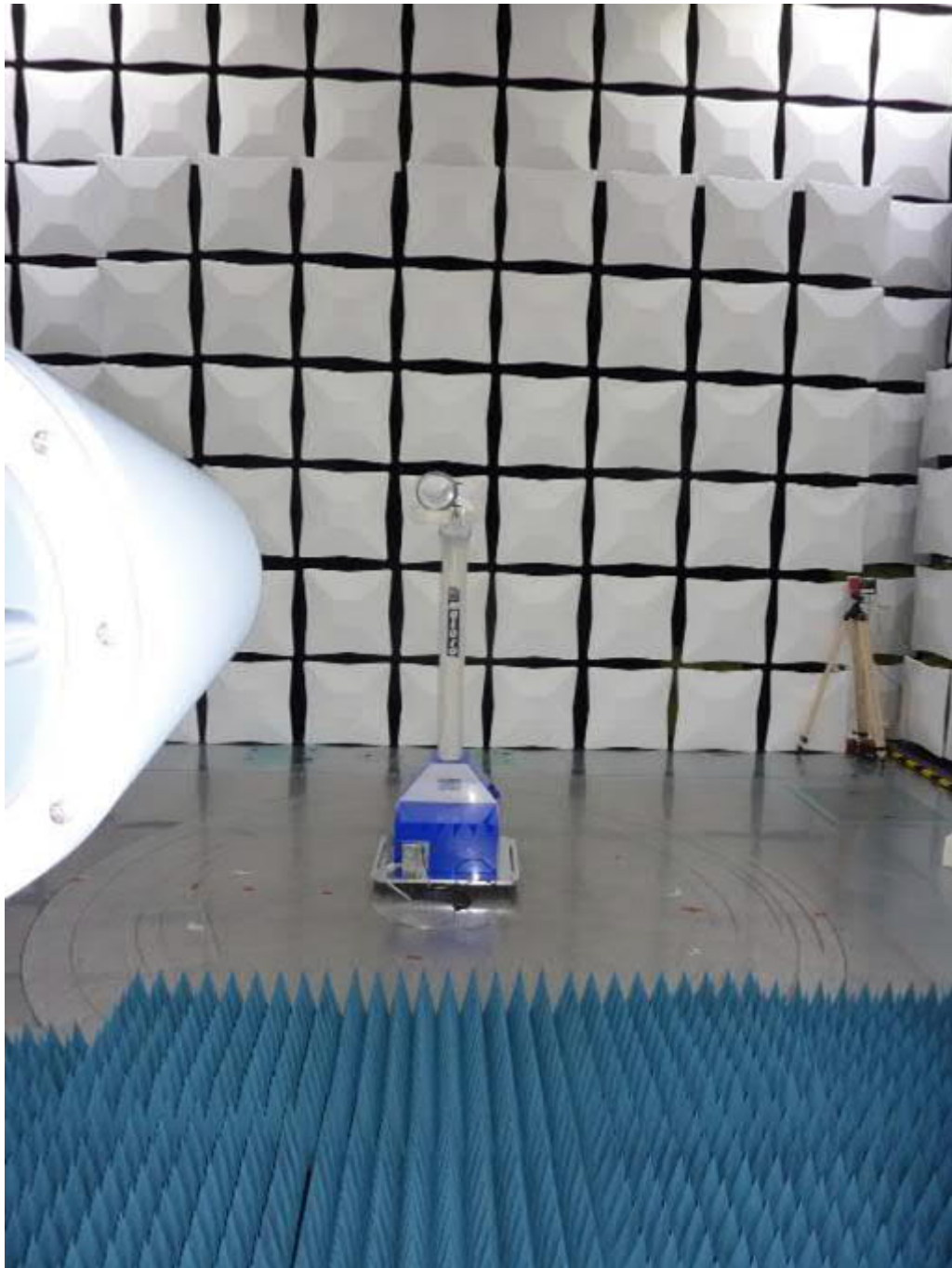
WS800-UMB, test setup fully anechoic chamber
