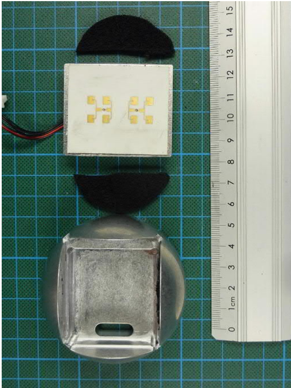
WS800-UMB, radar modul carrier, module removed
