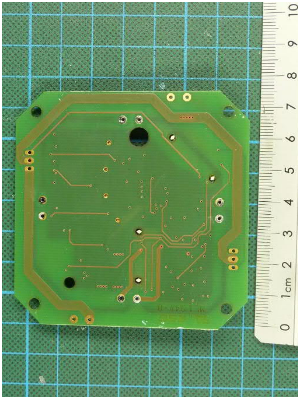
WS800-UMB, ultra sonic PCB, bottom view
