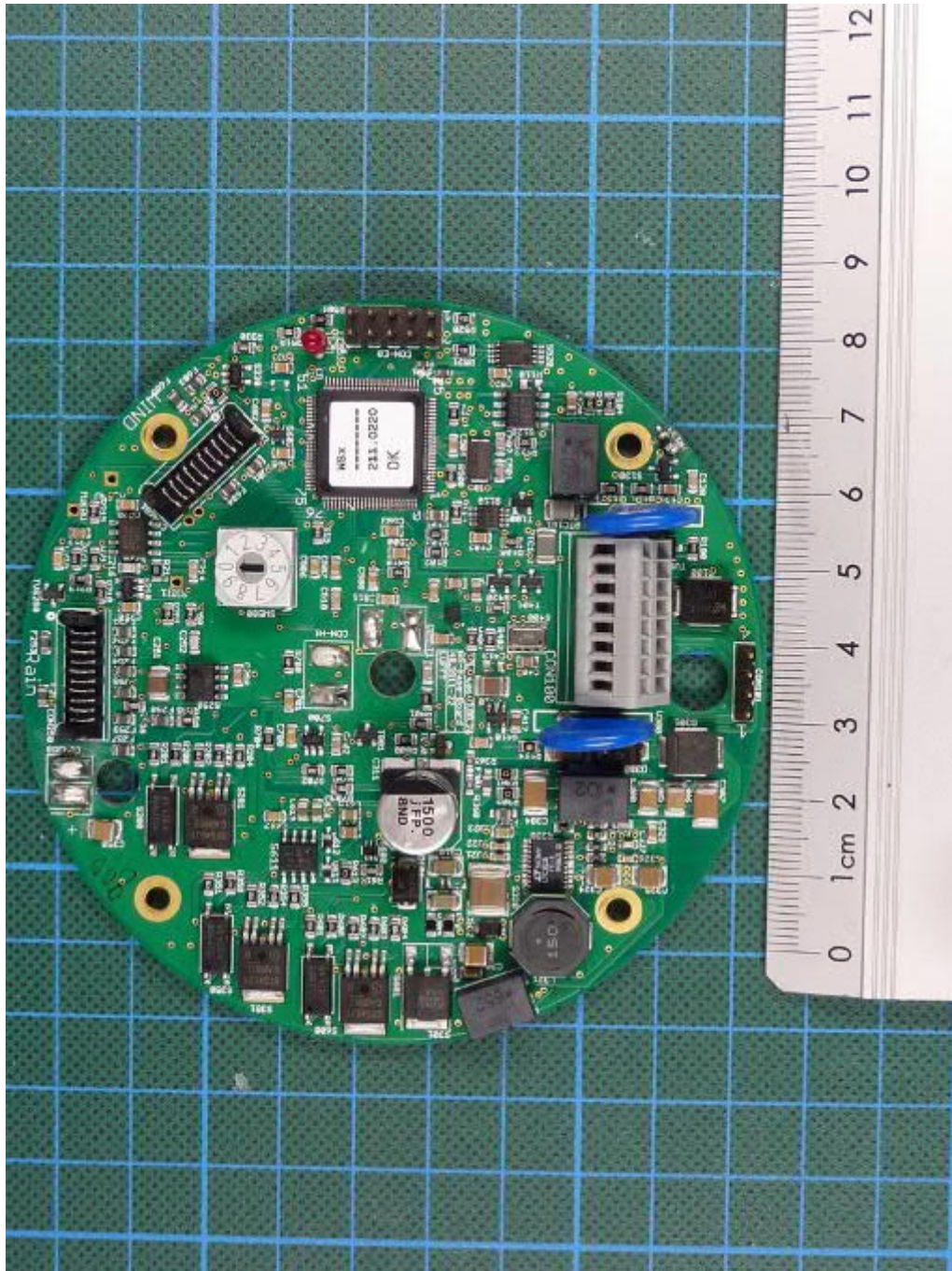
WS800-UMB, main PCB, top view
