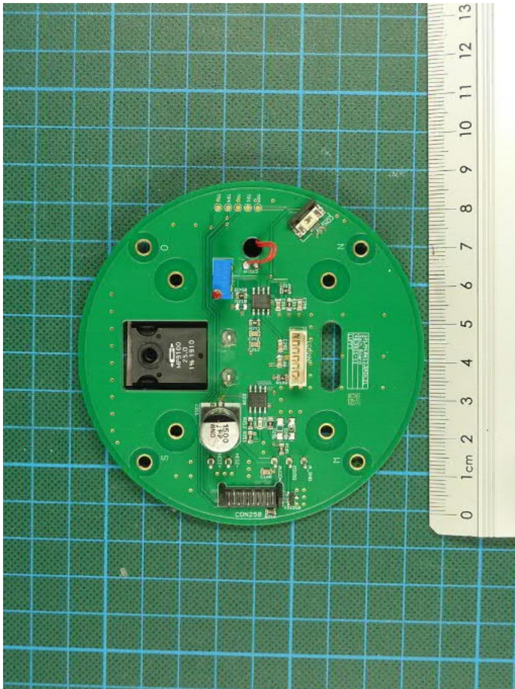
WS800-UMB, radar carrier PCB, top view
