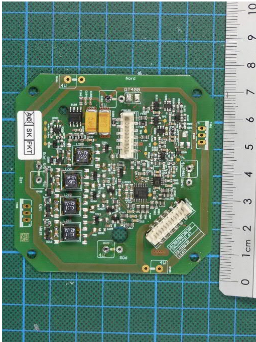
WS800-UMB, ultra sonic PCB, top view
