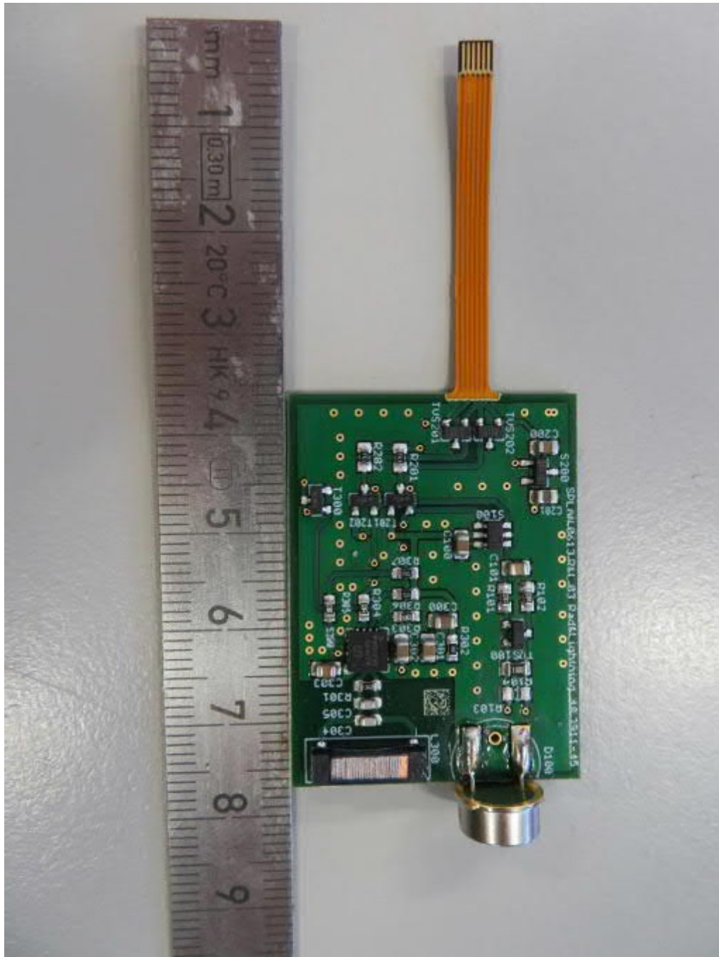
WS800-UMB, lightning sensor PCB, top view (supplied by the applicant)
