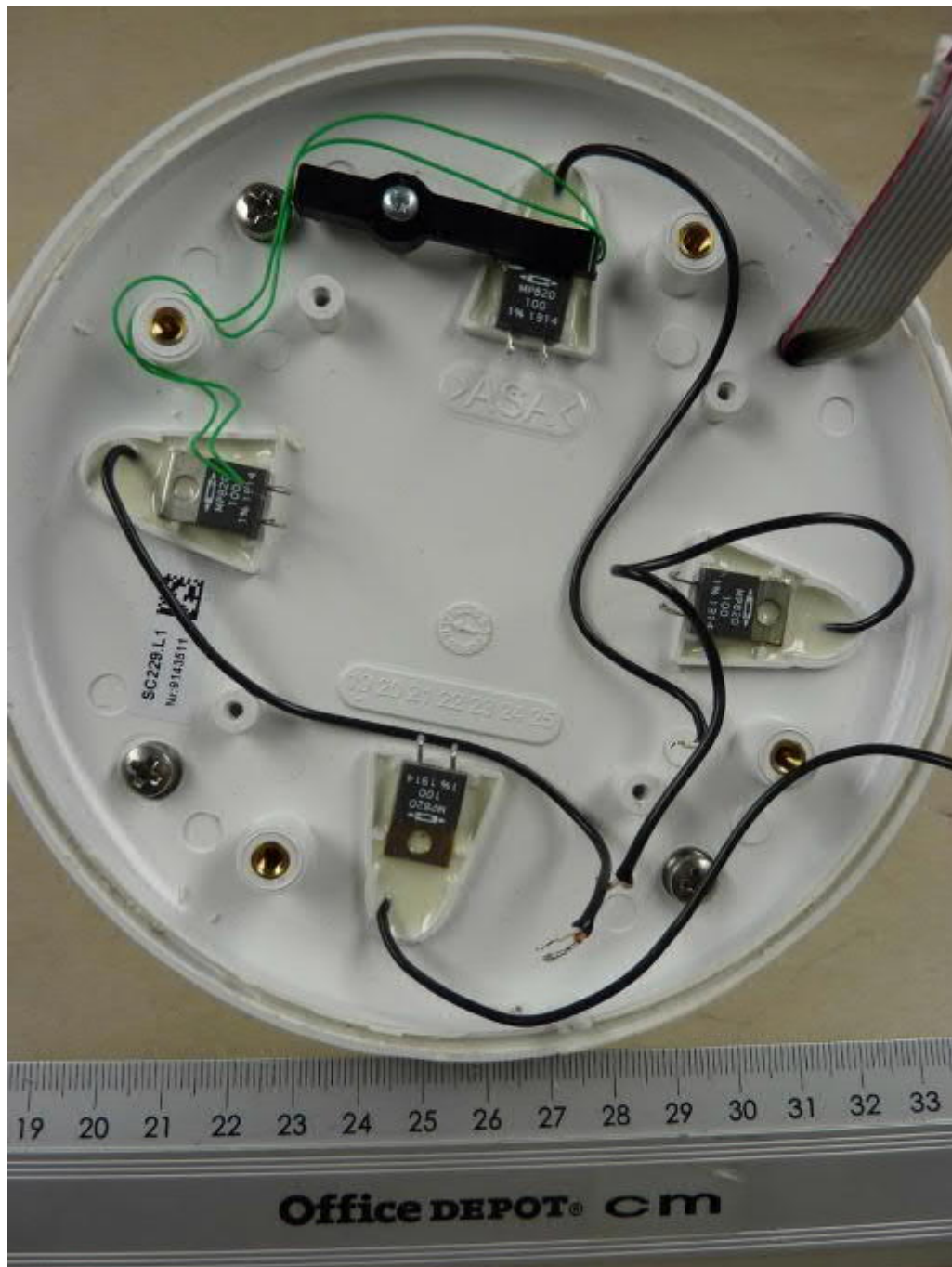
WS800-UMB, housing, ultra sonic PCB removed
