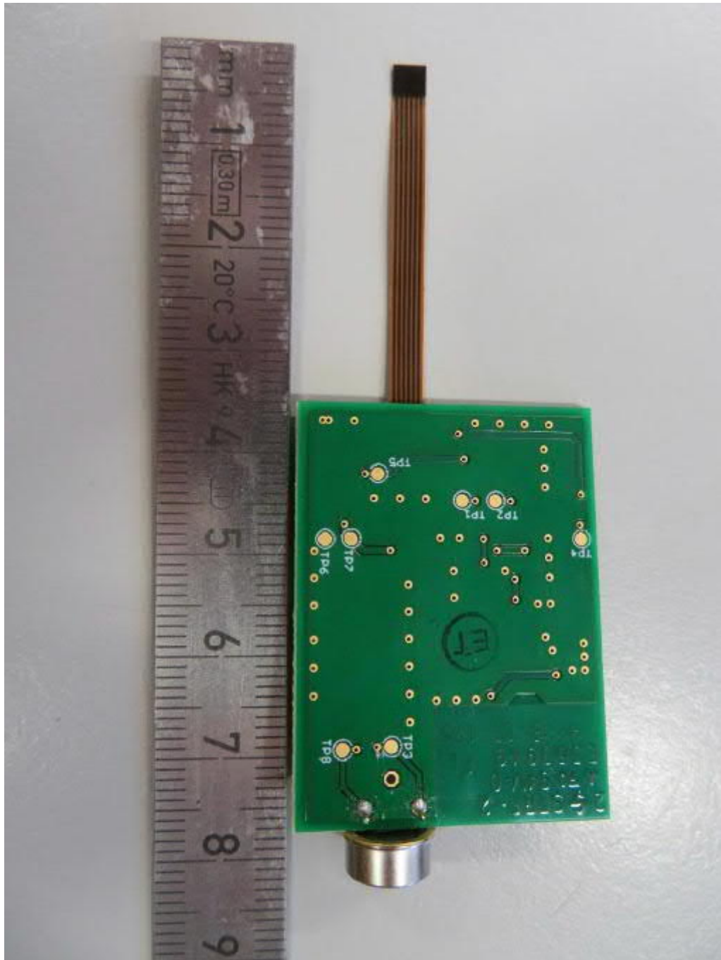
WS800-UMB, lightning sensor PCB, bottom view (supplied by the applicant)
