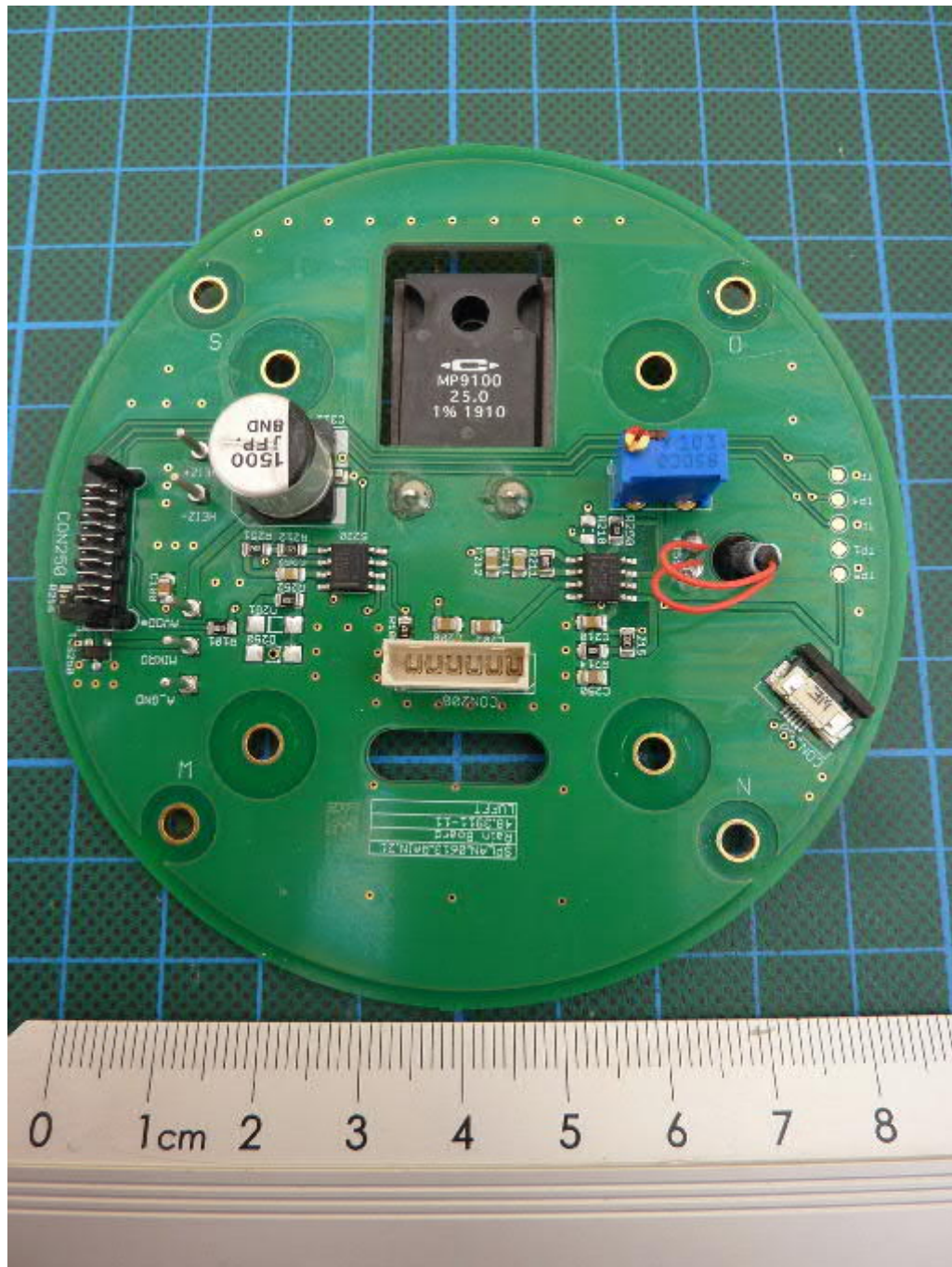
WS700-UMB, radar carrier PCB, top view
