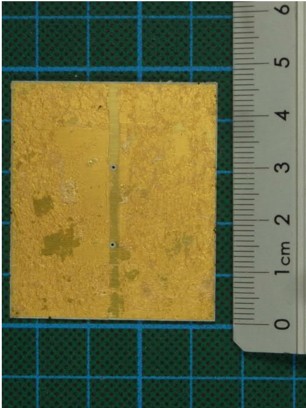
WS400-UMB, radar module, antenna PCB, bottom view
