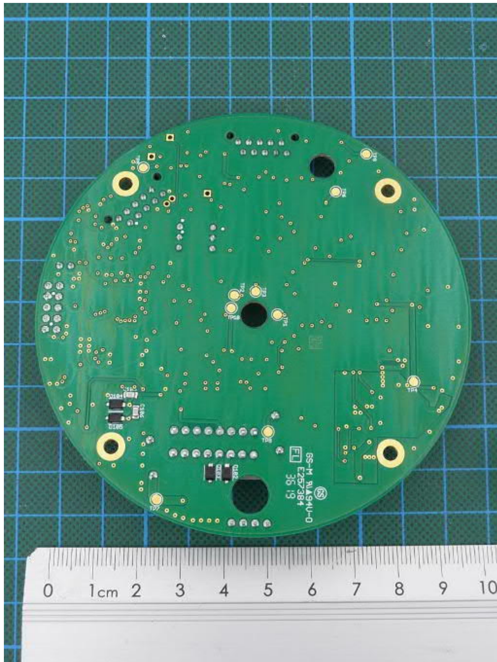
WS400-UMB, main PCB, bottom view
