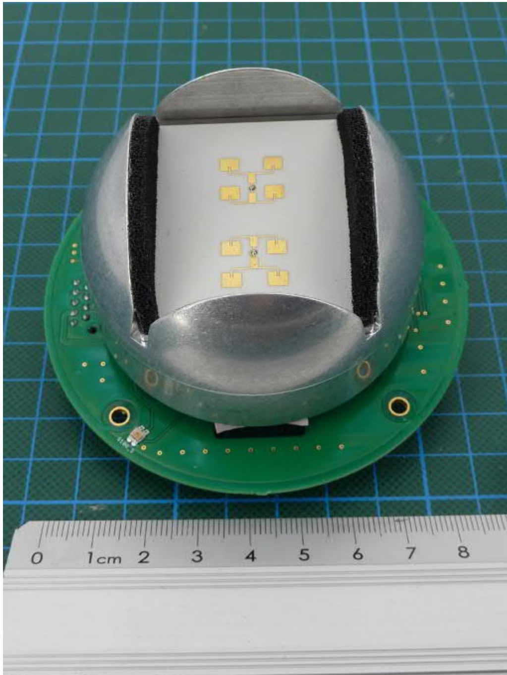
WS400-UMB, radar part, total view
