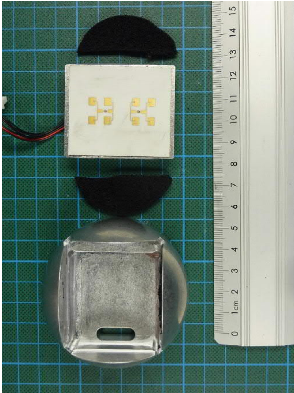
WS400-UMB, radar modul carrier, module removed
