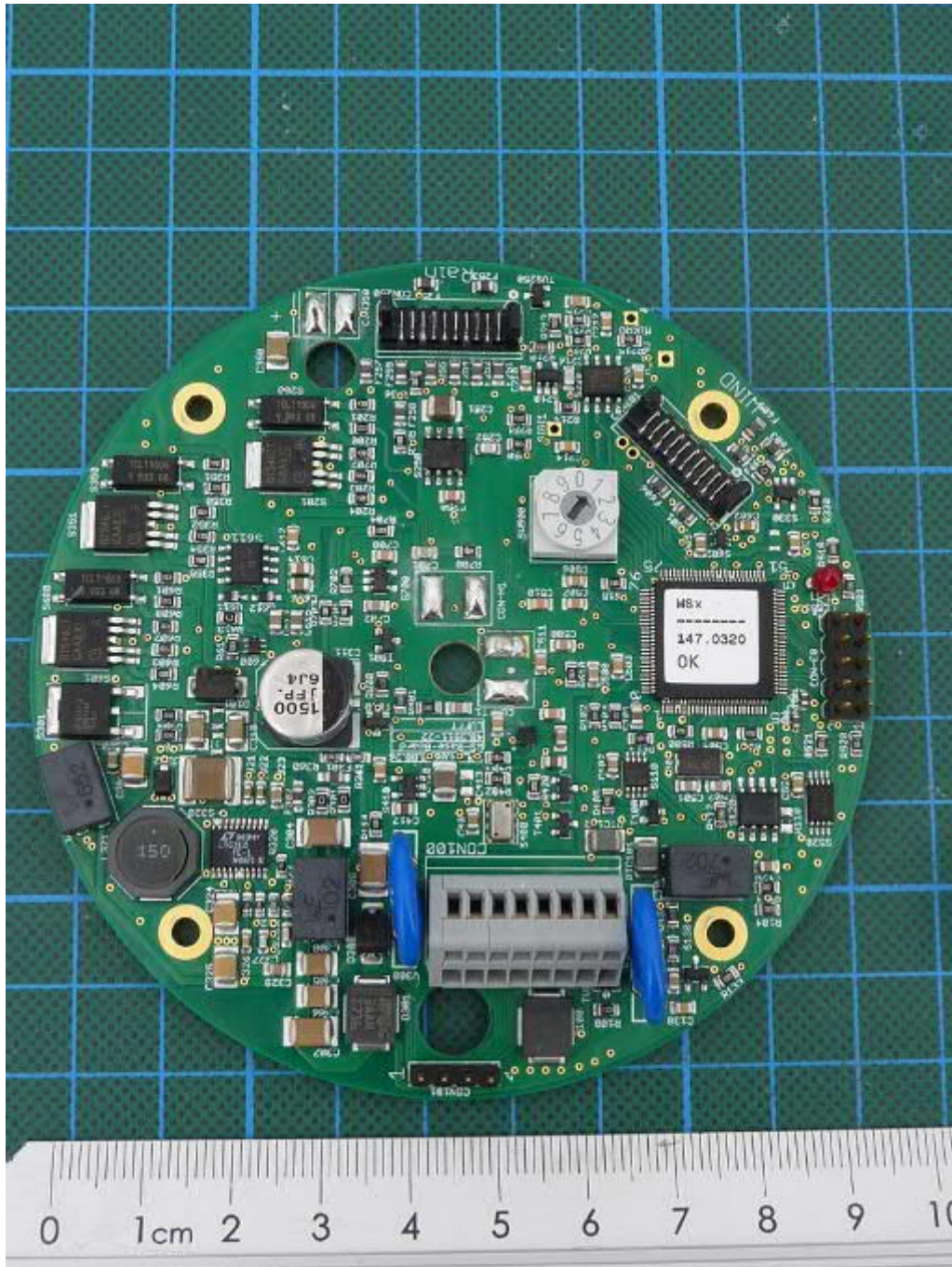
WS400-UMB, main PCB, top view
