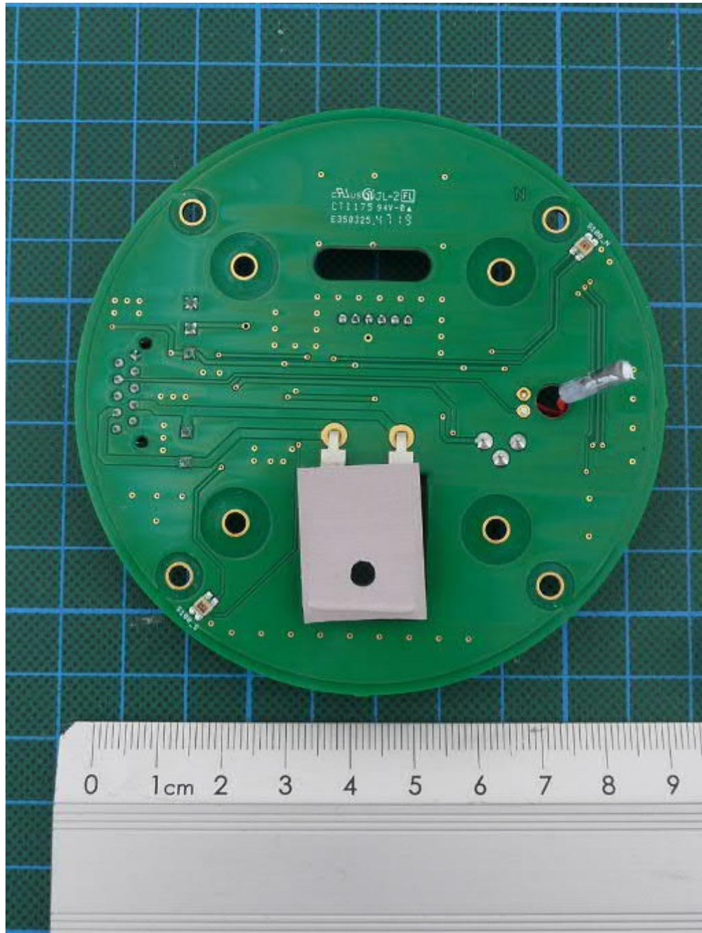
WS400-UMB, radar carrier PCB, bottom view
