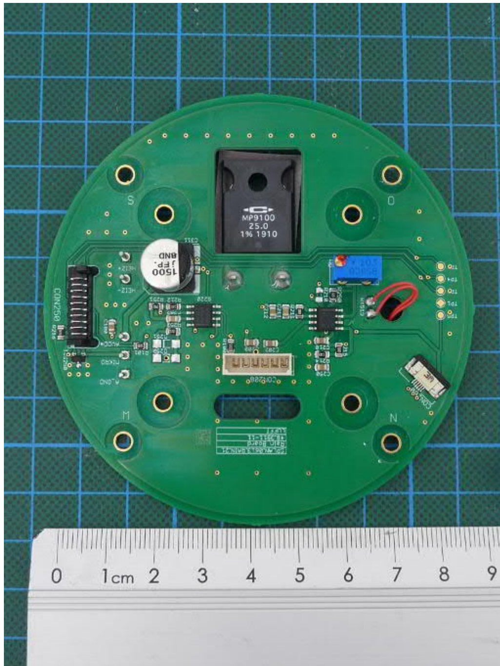
WS400-UMB, radar carrier PCB, top view
