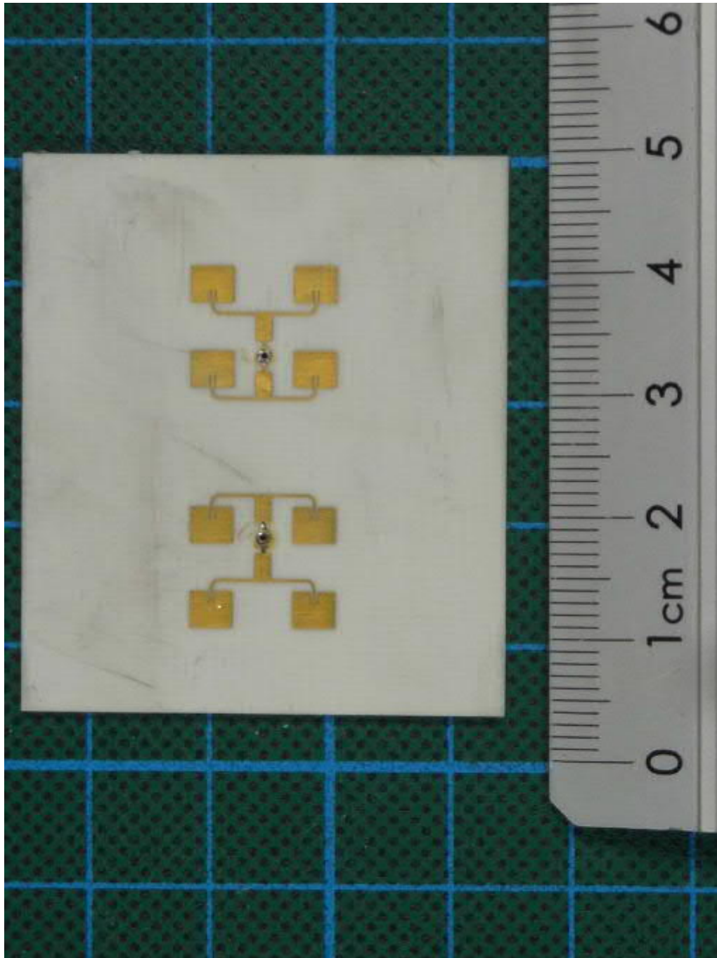
WS400-UMB, radar module, antenna PCB, top view
