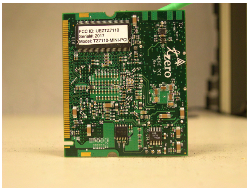
Figure 2. Reverse side of Tzero TZ7110 Mini-PCI adaptor including ID label.
