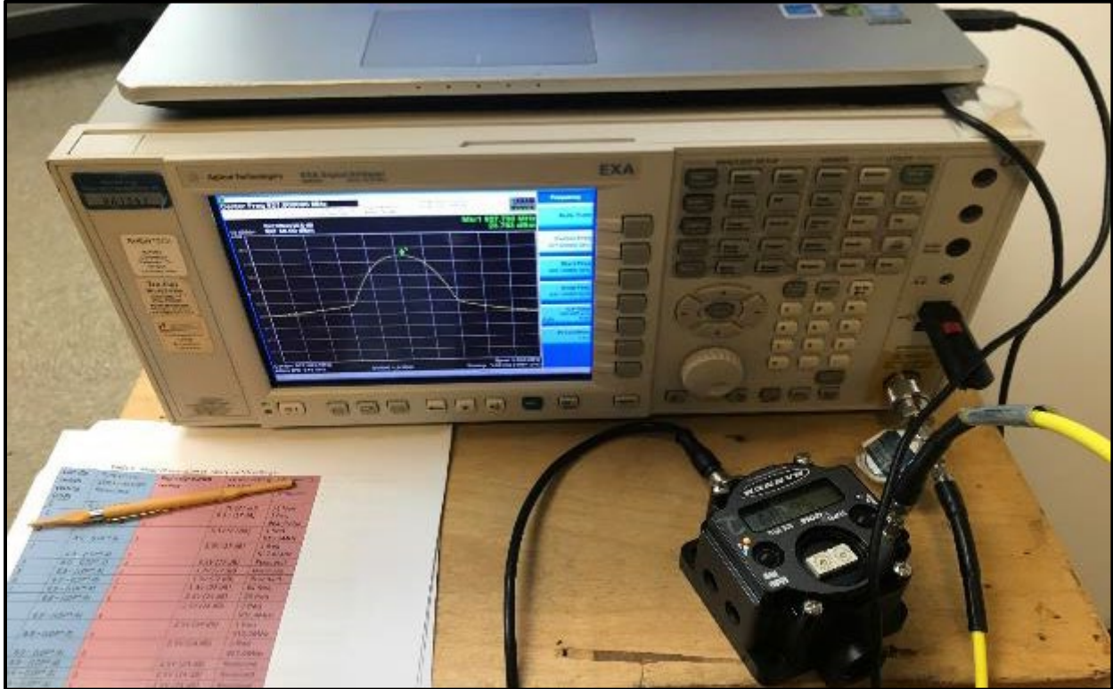
Photograph 1: Conducted Emissions Test Setup
