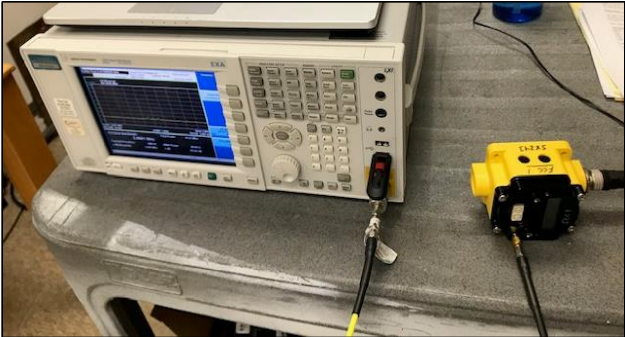
Photograph 4: Conducted Emissions Test Setup
