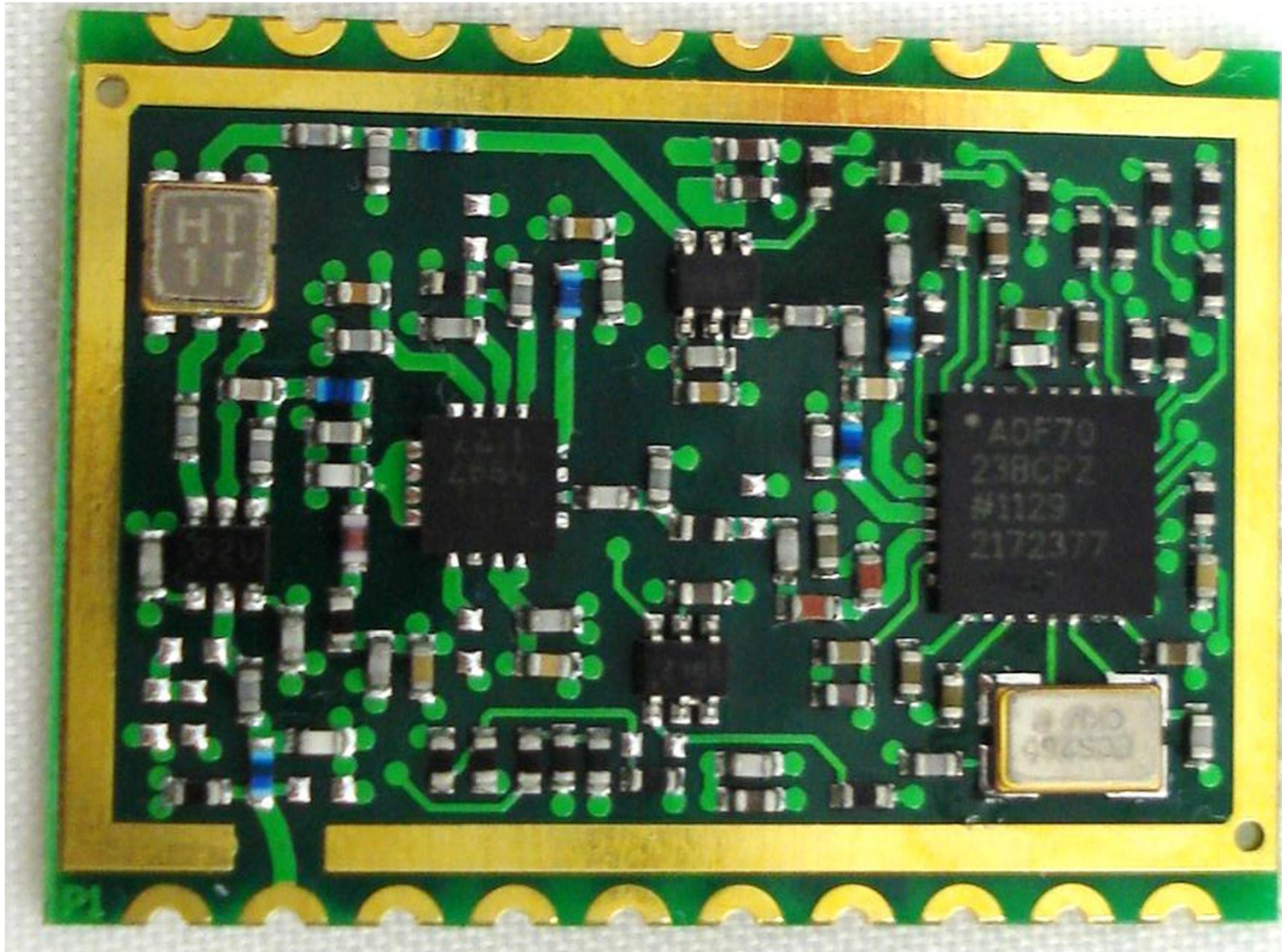
Front side of RM7023
