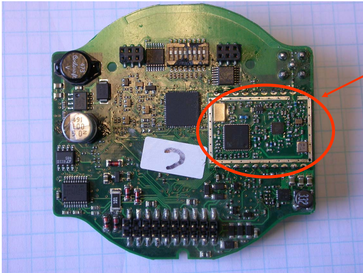
Front side of DX180 with shield off of RM1809
