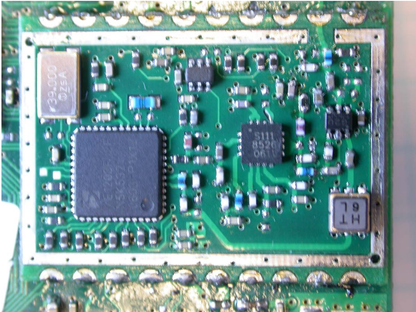
Front side of RM1809
