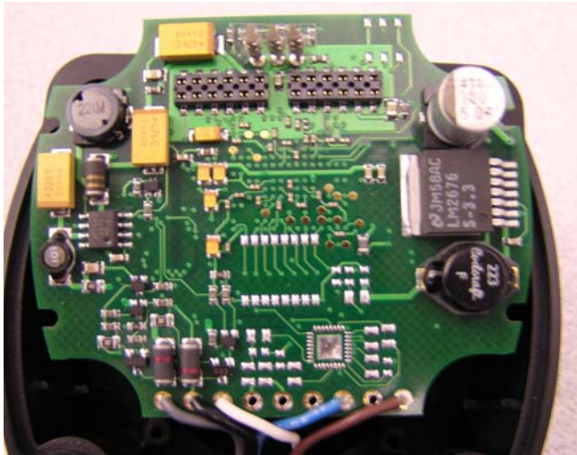
PCB ASSEMBLY 121950 / PCB ASSY FPGA/POWER/OUTPUT
