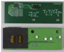
Figure 6, PCB Assy 153597
