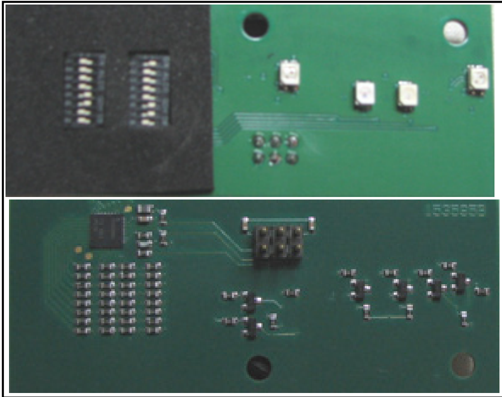
Photograph 10: Display Board – Front and Back Views
