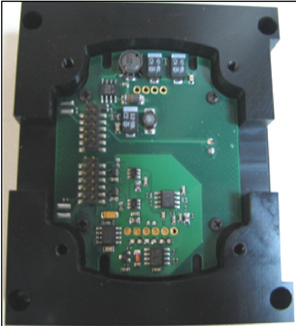
Photograph 6: Amp Board
