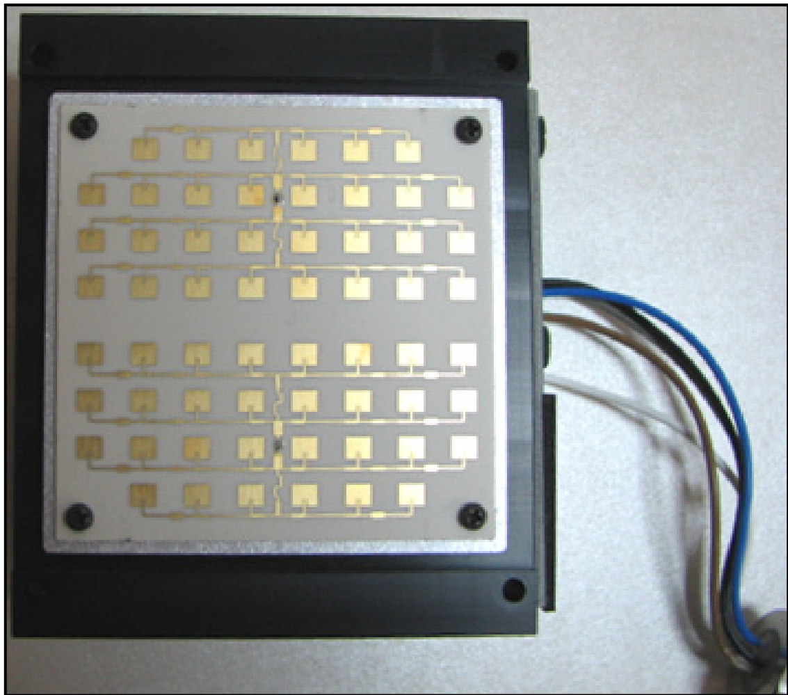
Photograph 4: Antenna on Top of Block
