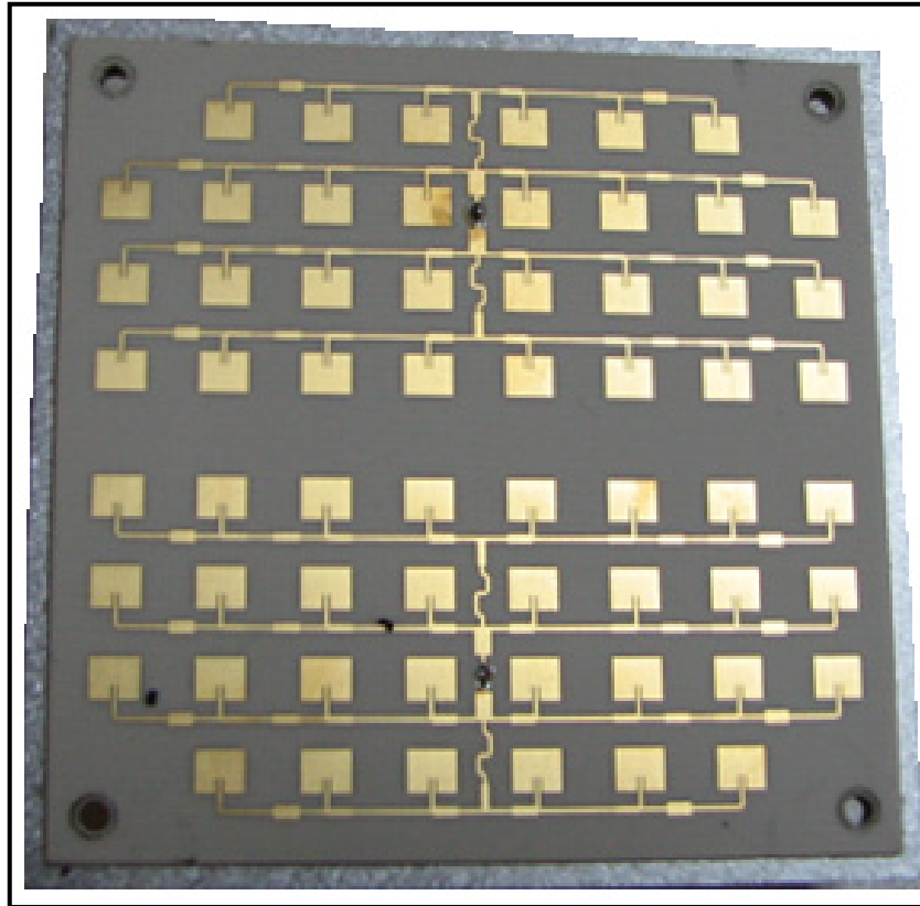
Photograph 11: Radar Module - Front View
