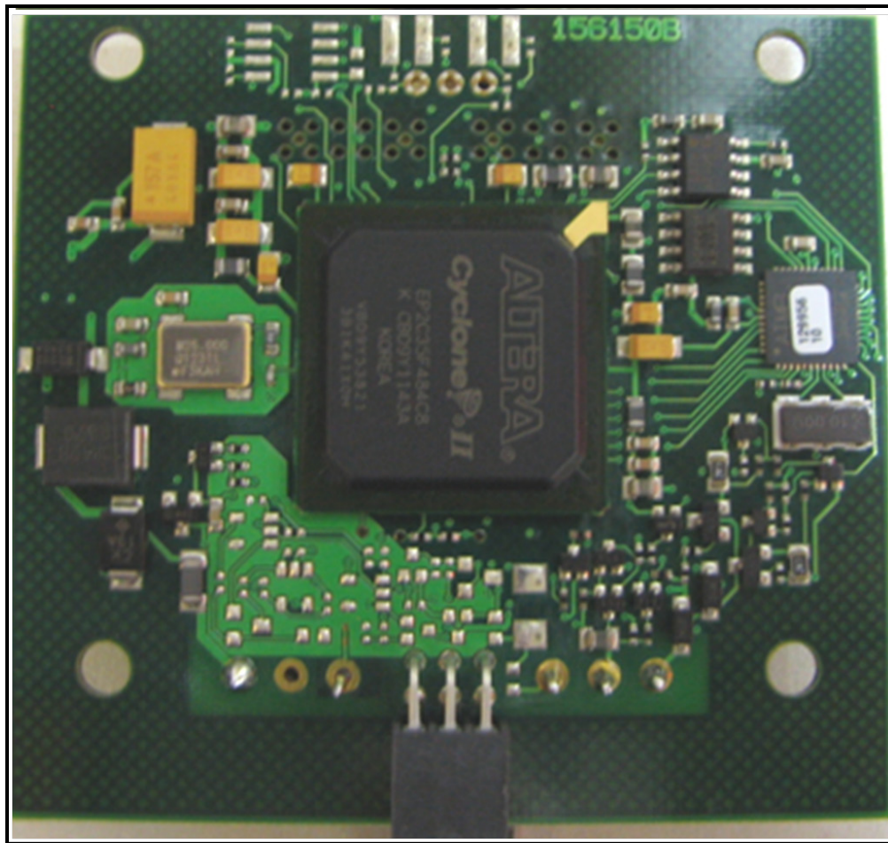
Photograph 8: FPGA Board Side 1
