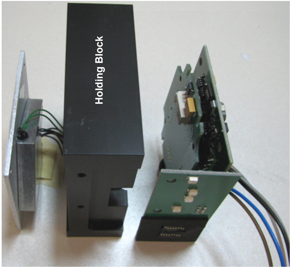
Photograph 3: Internal Modules
