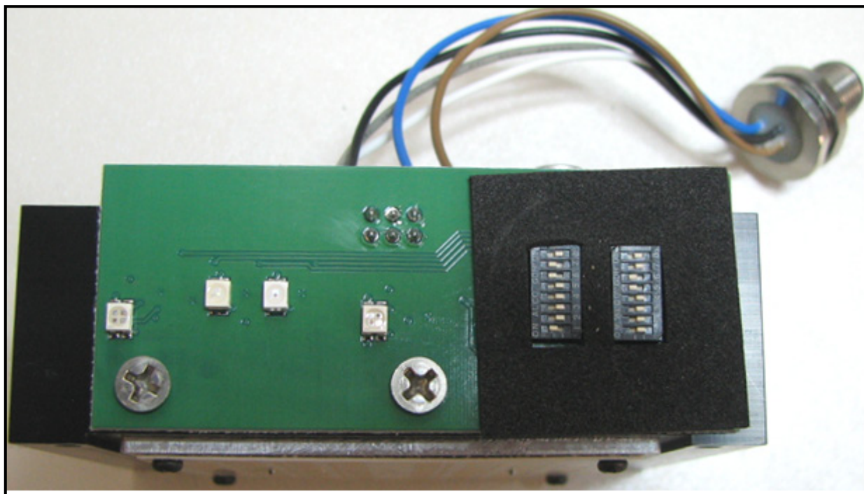
Photograph 5: User Interface Board on Side of Block
