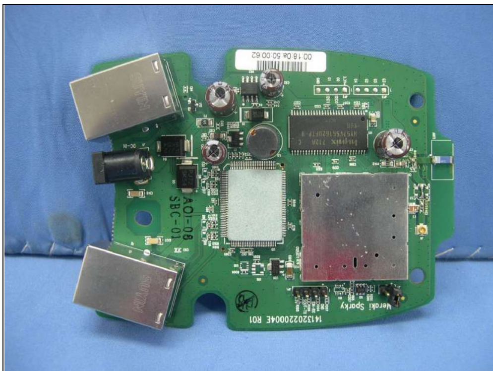
Antenna Model No.: RFANT5220110A0T
