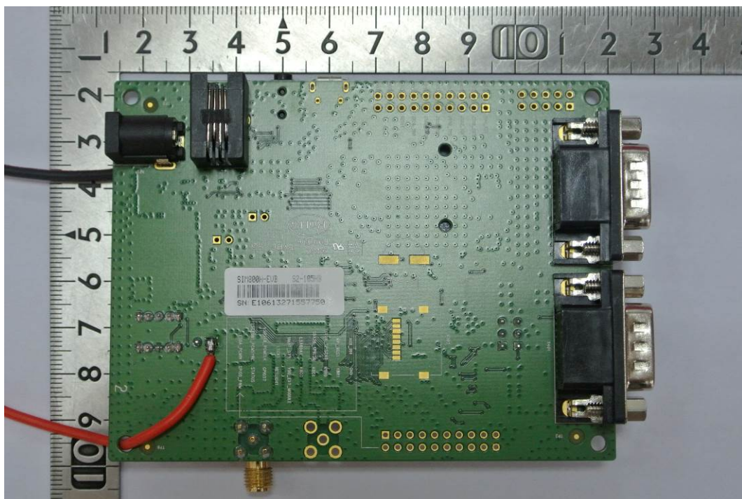
Bottom View with EVB
