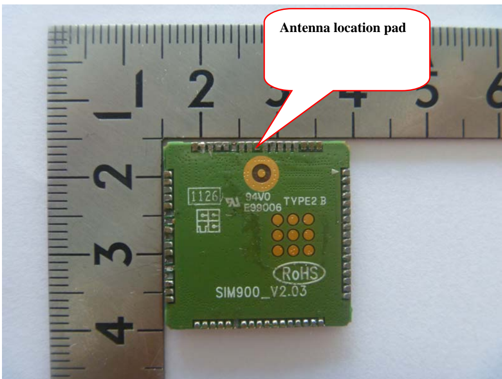
SIM900L_Back View
