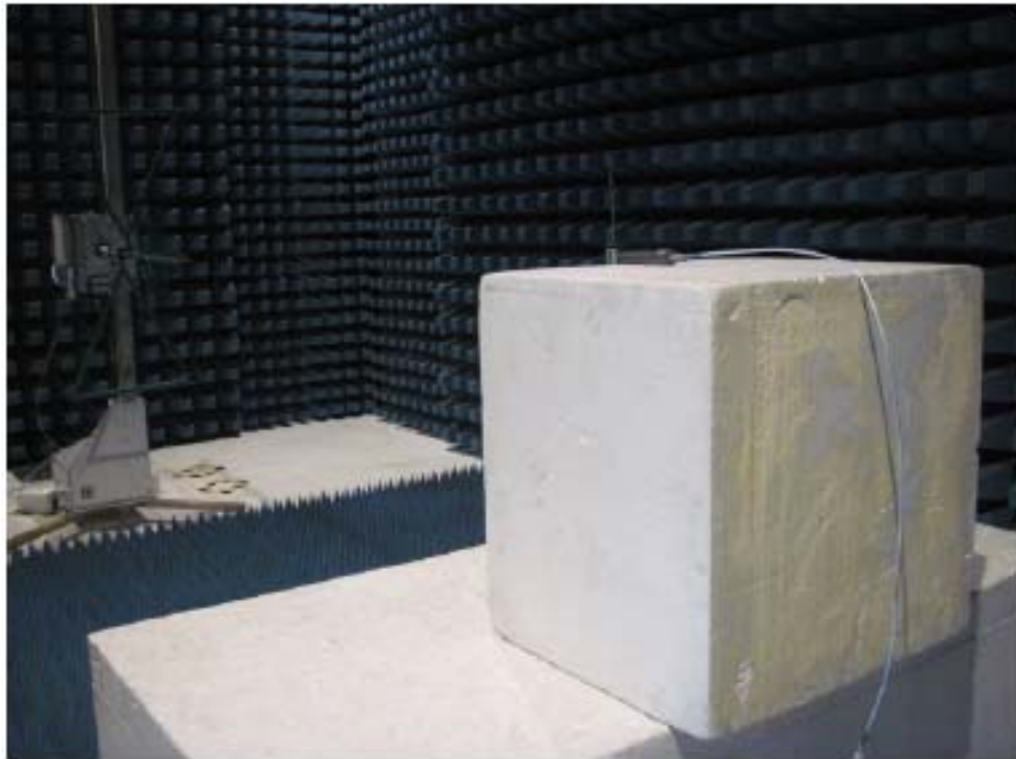
Spurious Emission/ERP Test:
