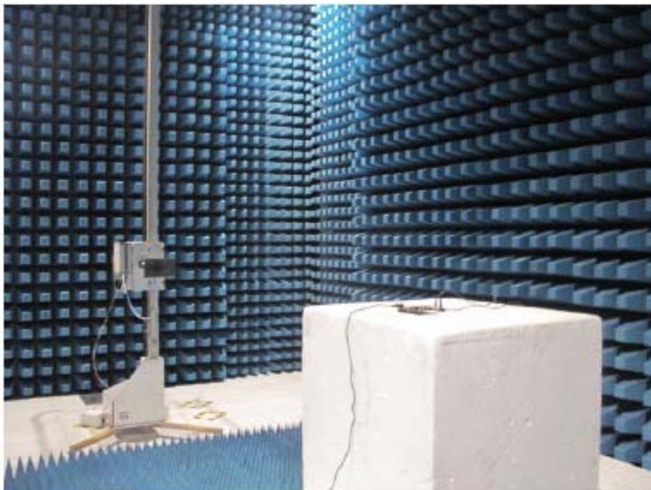
Spurious Emission/EIRP Test
