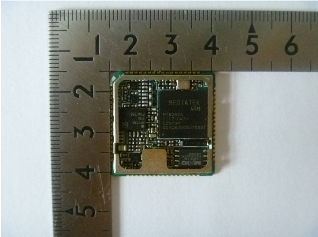
Top View
