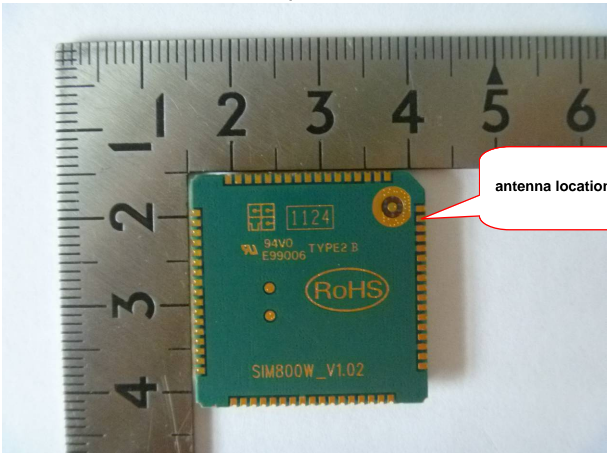
Bottom View
