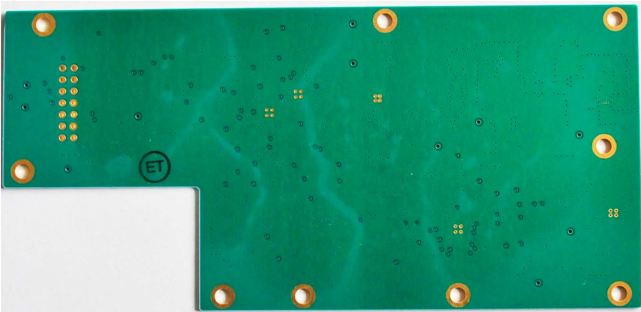
Figure E23.4 – Internal – Up / Down Converters, Bottom Side
