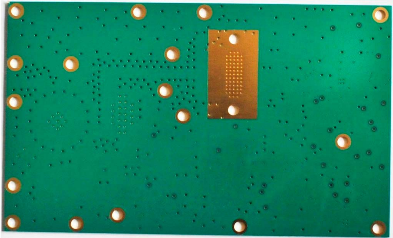
Figure E23.6 – Internal – Power Amplifier, Bottom Side
