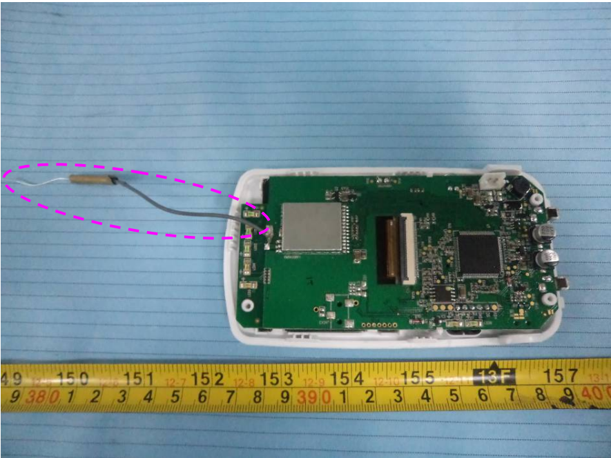
EUT – AntennaView
