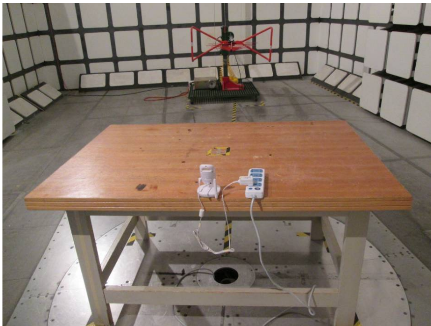
Radiated Emissions –Rear View (Below 1 GHz for KINGS adater)
