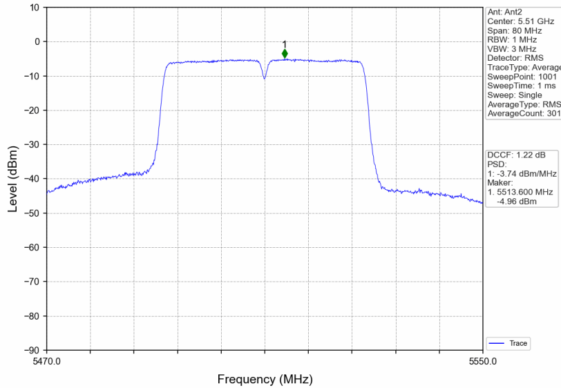
802.11ac(VHT40)_LCH_5510MHz_MIMO_NTNV
