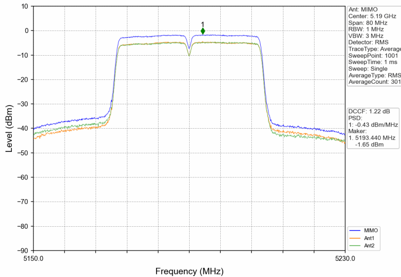
802.11ac(VHT40)_LCH_5190MHz_MIMO_NTNV
