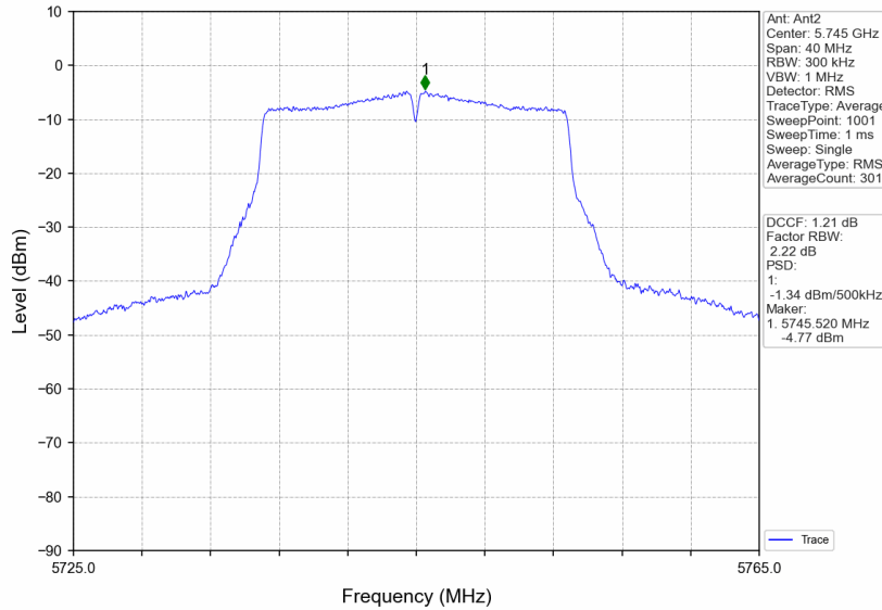
802.11ac(VHT20)_LCH_5745MHz_MIMO_NTNV
