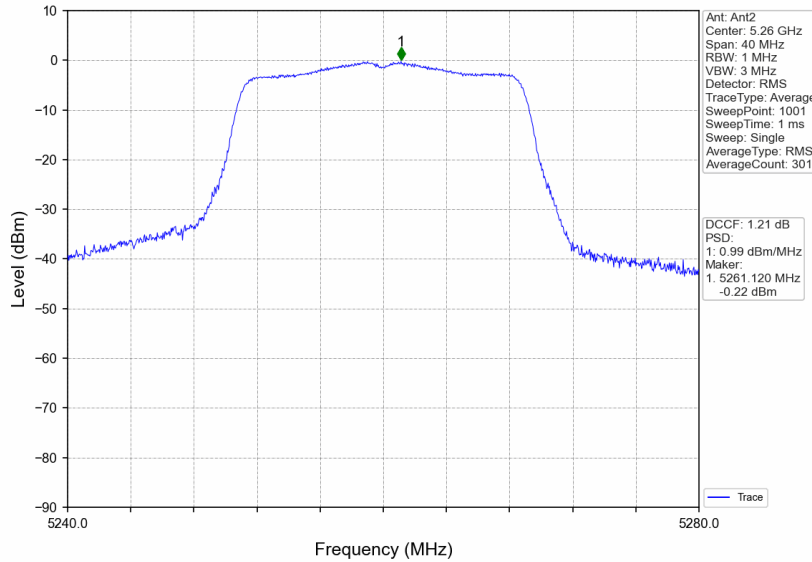
802.11n(HT20)_LCH_5260MHz_MIMO_NTNV
