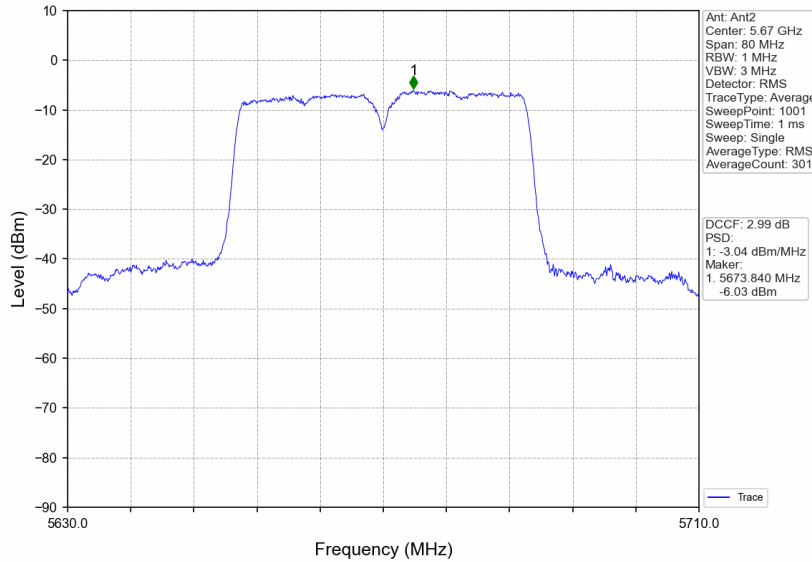
802.11n(HT40)_HCH_5670MHz_MIMO_NTNV
