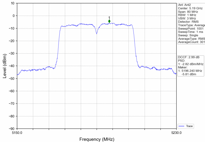
802.11n(HT40)_LCH_5190MHz_MIMO_NTNV
