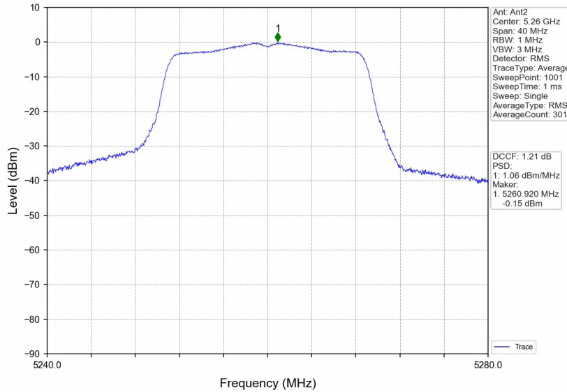
802.11ac(VHT20)_LCH_5260MHz_MIMO_NTNV
