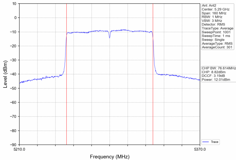
802.11ac(VHT80)_MCH_5290MHz_Ant2_NTNV
