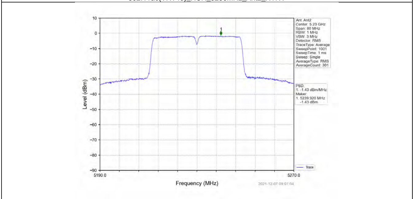
802.11ac(VHT40)_HCH_5230MHz_MIMO_NTNV
