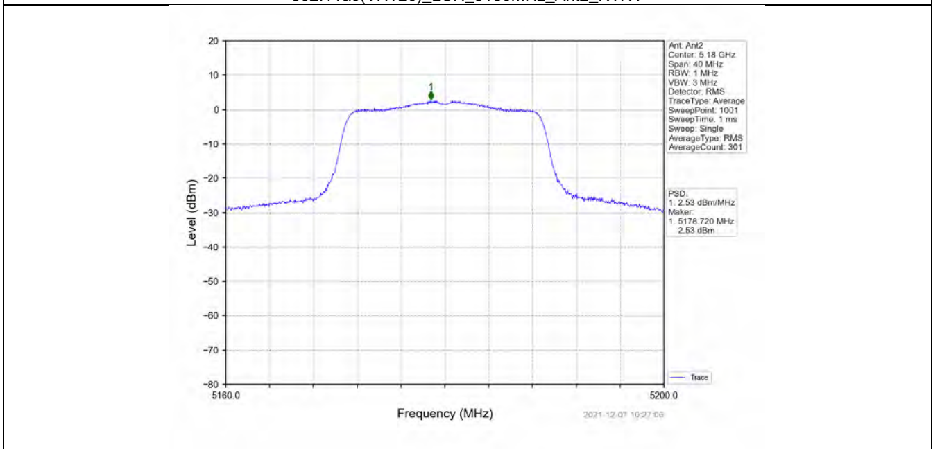
802.11ac(VHT20)_LCH_5180MHz_MIMO_NTNV
