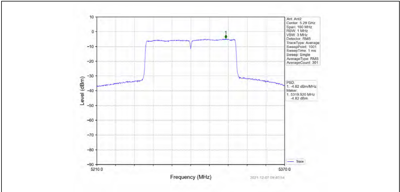
802.11ac(VHT80)_MCH_5290MHz_MIMO_NTNV
