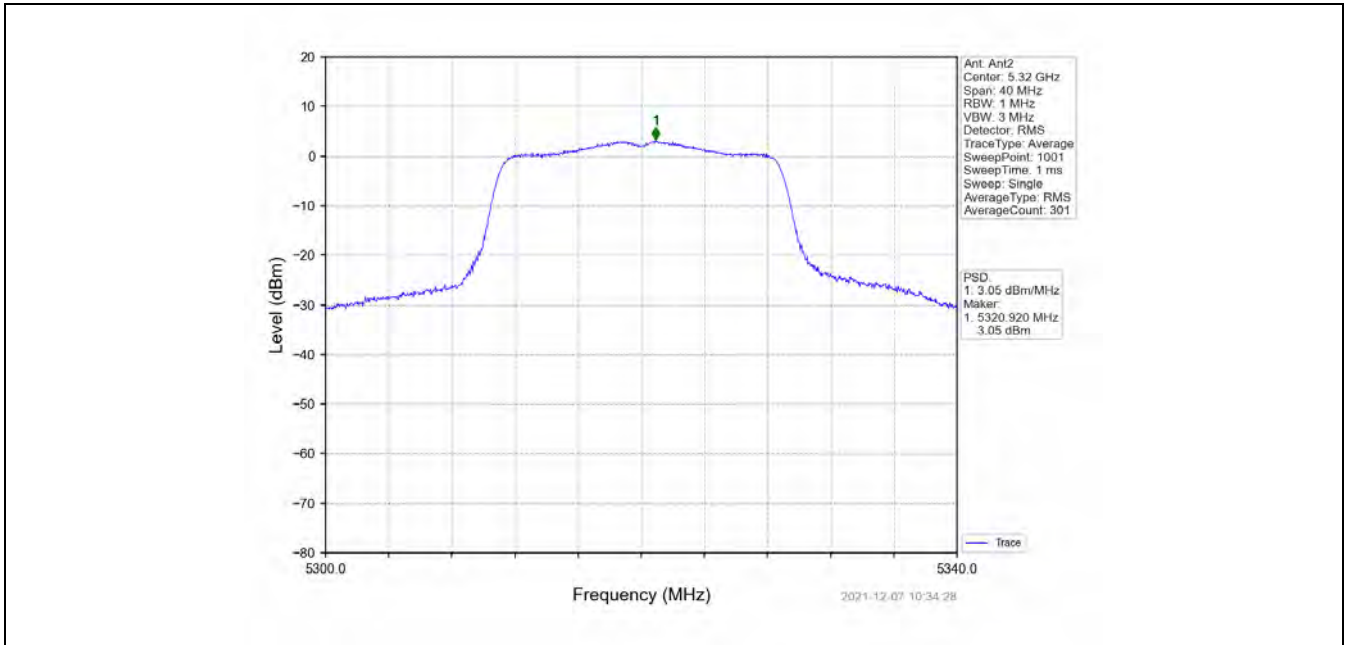
802.11ac(VHT20)_HCH_5320MHz_MIMO_NTNV
