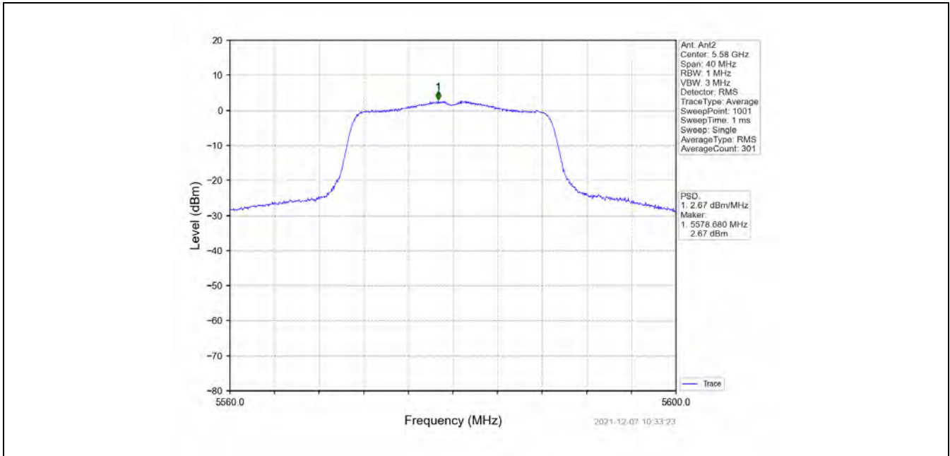
802.11ac(VHT20)_MCH_5580MHz_MIMO_NTNV
