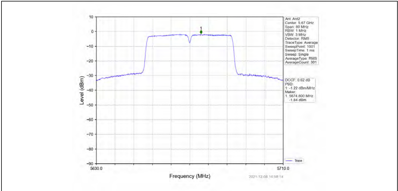
802.11n(HT40)_HCH_5670MHz_MIMO_NTNV
