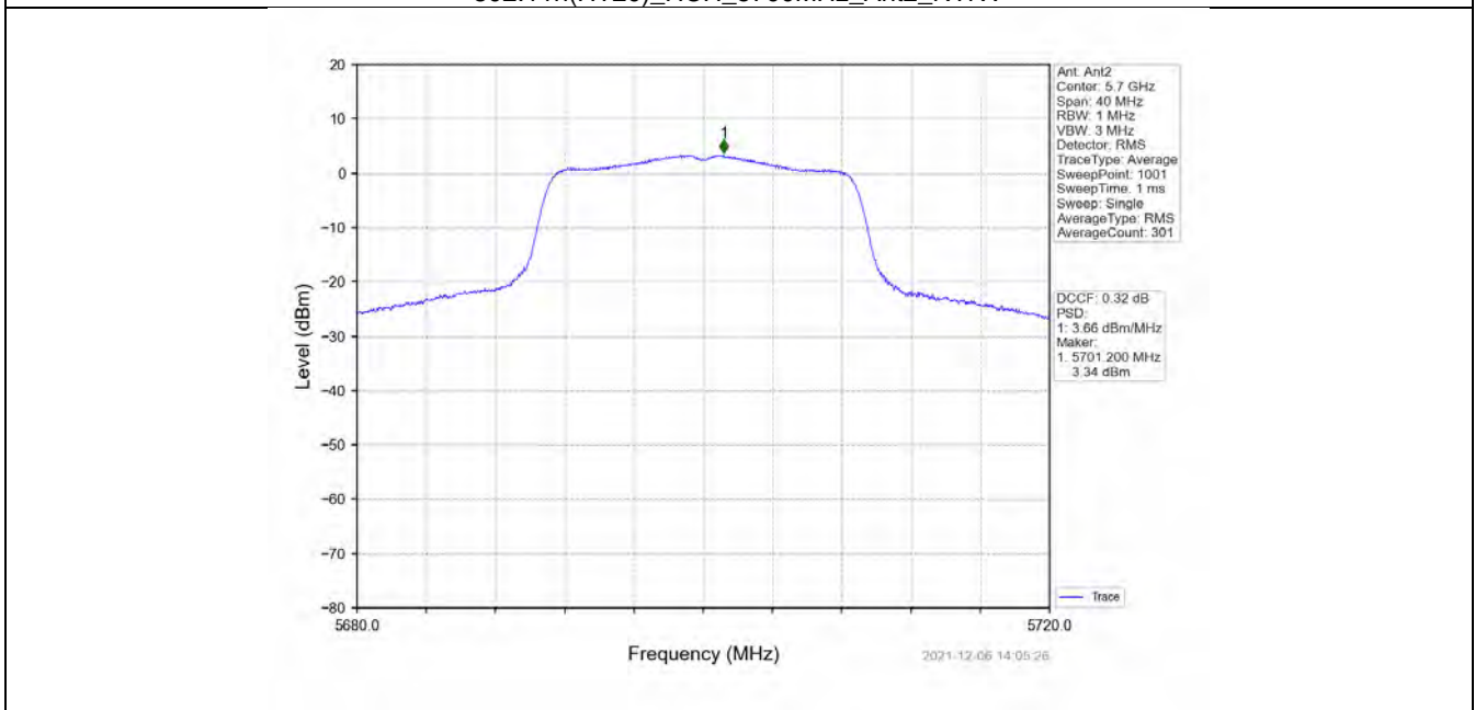
802.11n(HT20)_HCH_5700MHz_MIMO_NTNV
