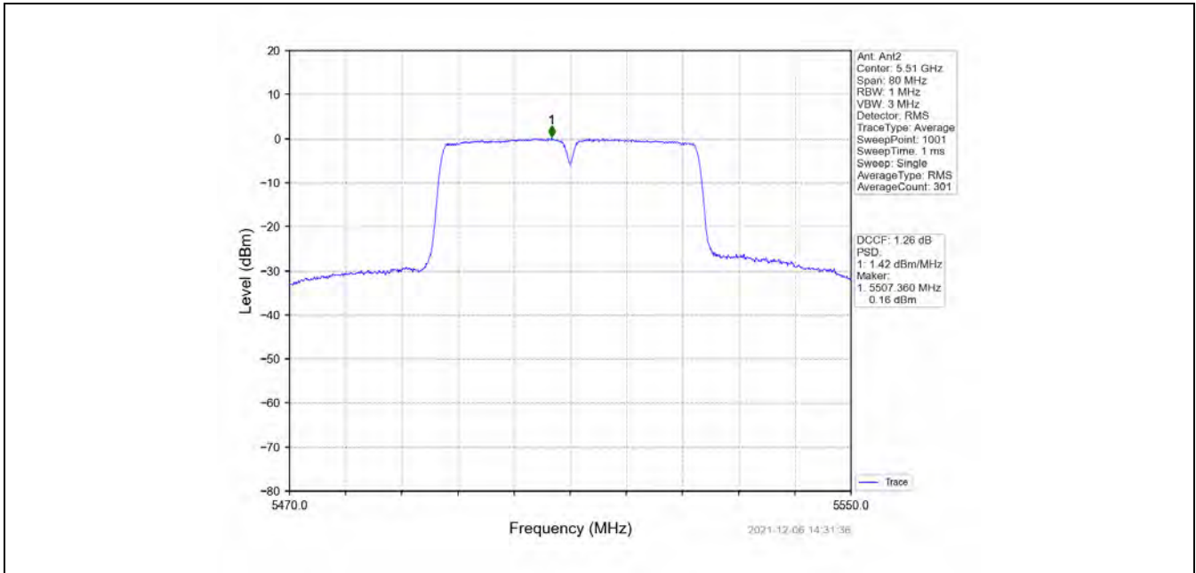
802.11n(HT40)_LCH_5510MHz_MIMO_NTNV
