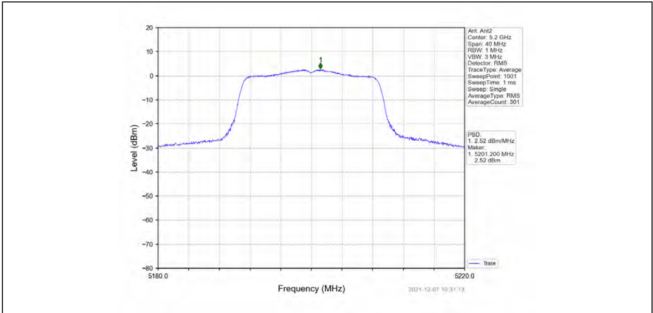
802.11ac(VHT20)_MCH_5200MHz_MIMO_NTNV
