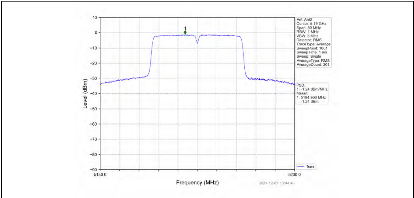
802.11ac(VHT40)_LCH_5190MHz_MIMO_NTNV
