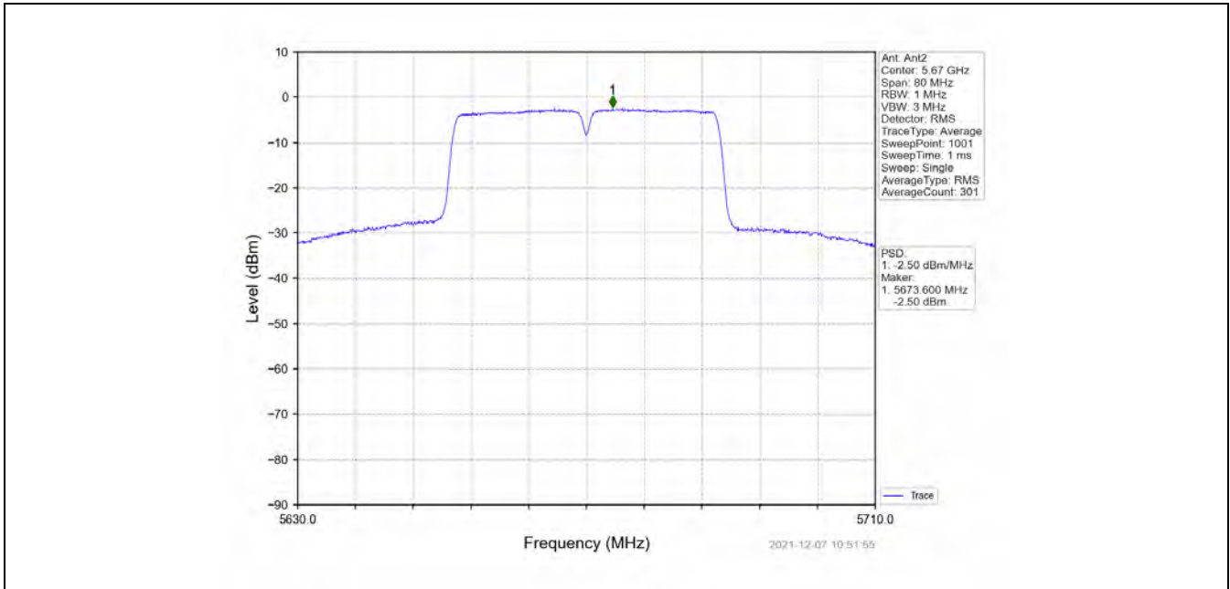
802.11ac(VHT40)_HCH_5670MHz_MIMO_NTNV
