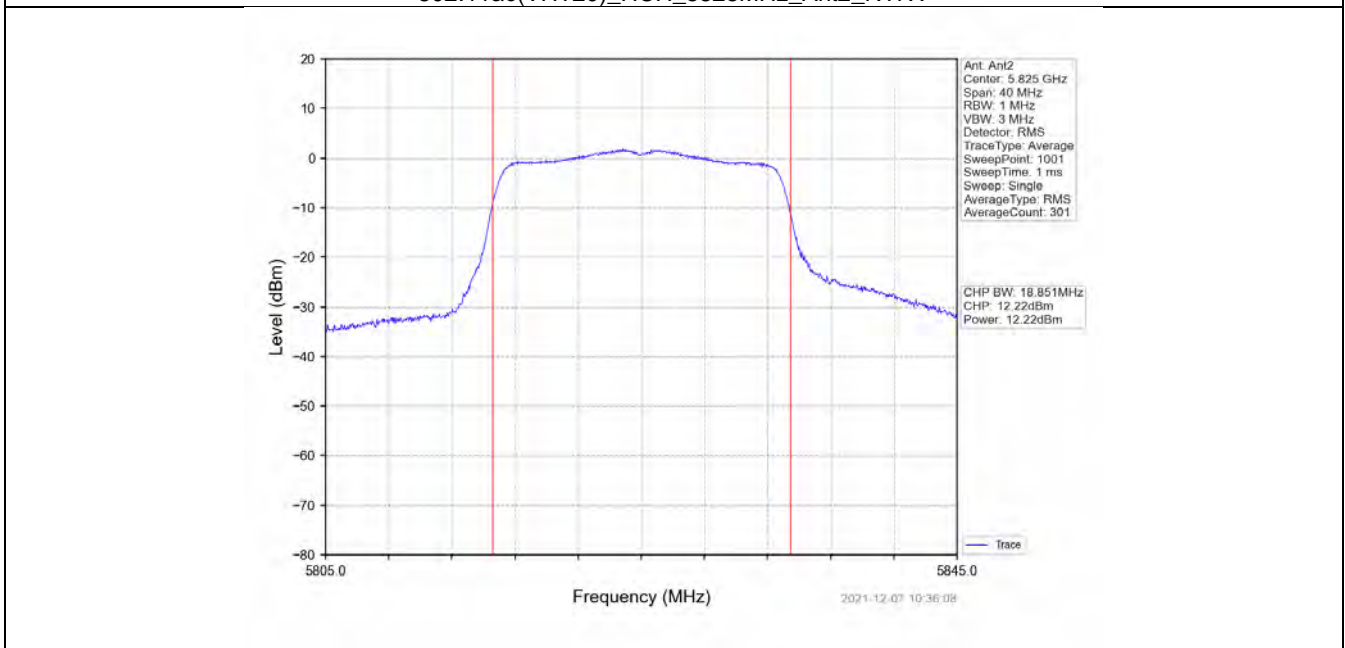
802.11ac(VHT40)_LCH_5190MHz_Ant1_NTNV
