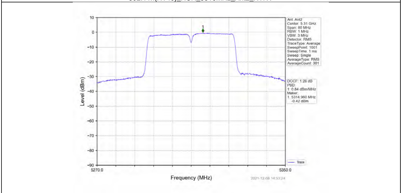
802.11n(HT40)_HCH_5310MHz_MIMO_NTNV
