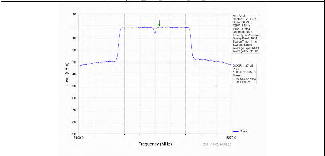
802.11n(HT40)_HCH_5230MHz_MIMO_NTNV
