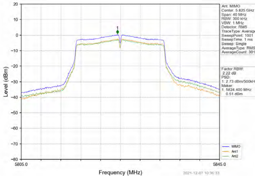
802.11ac(VHT20)_HCH_5825MHz_MIMO_NTNV
