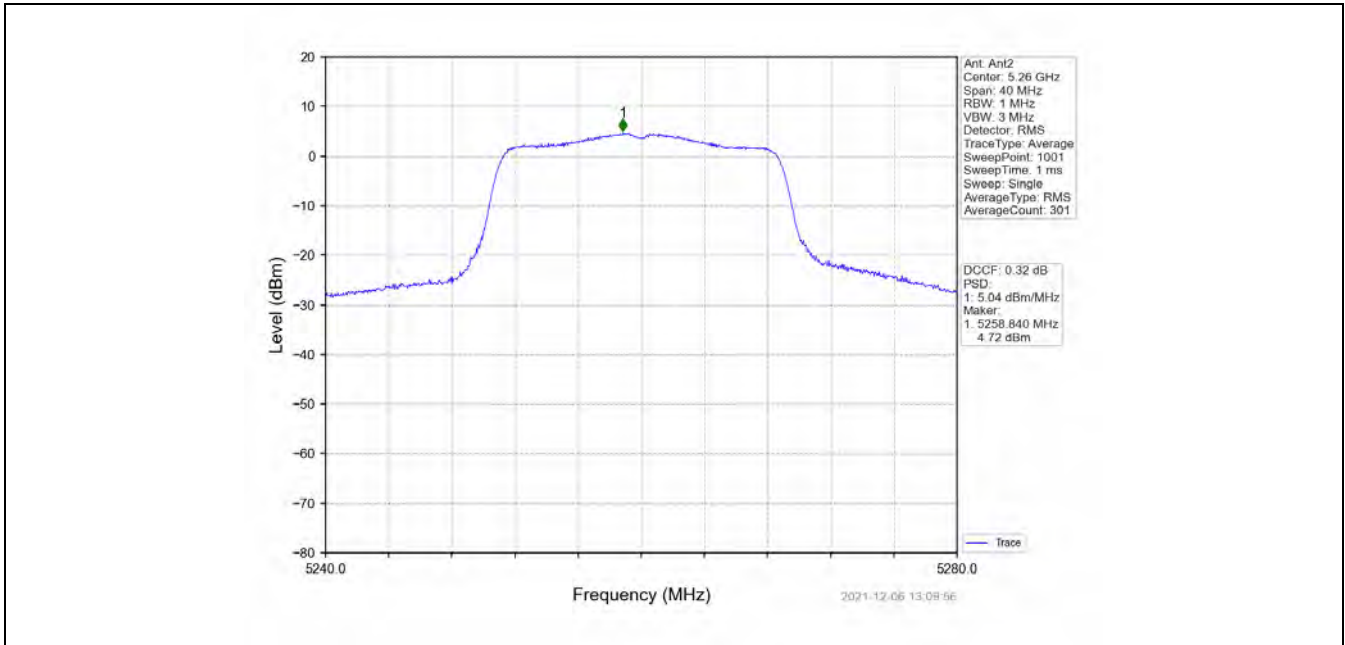
802.11n(HT20)_LCH_5260MHz_MIMO_NTNV
