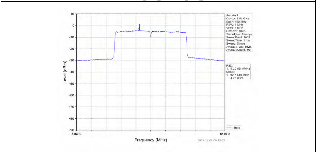
802.11ac(VHT80)_LCH_5530MHz_MIMO_NTNV
