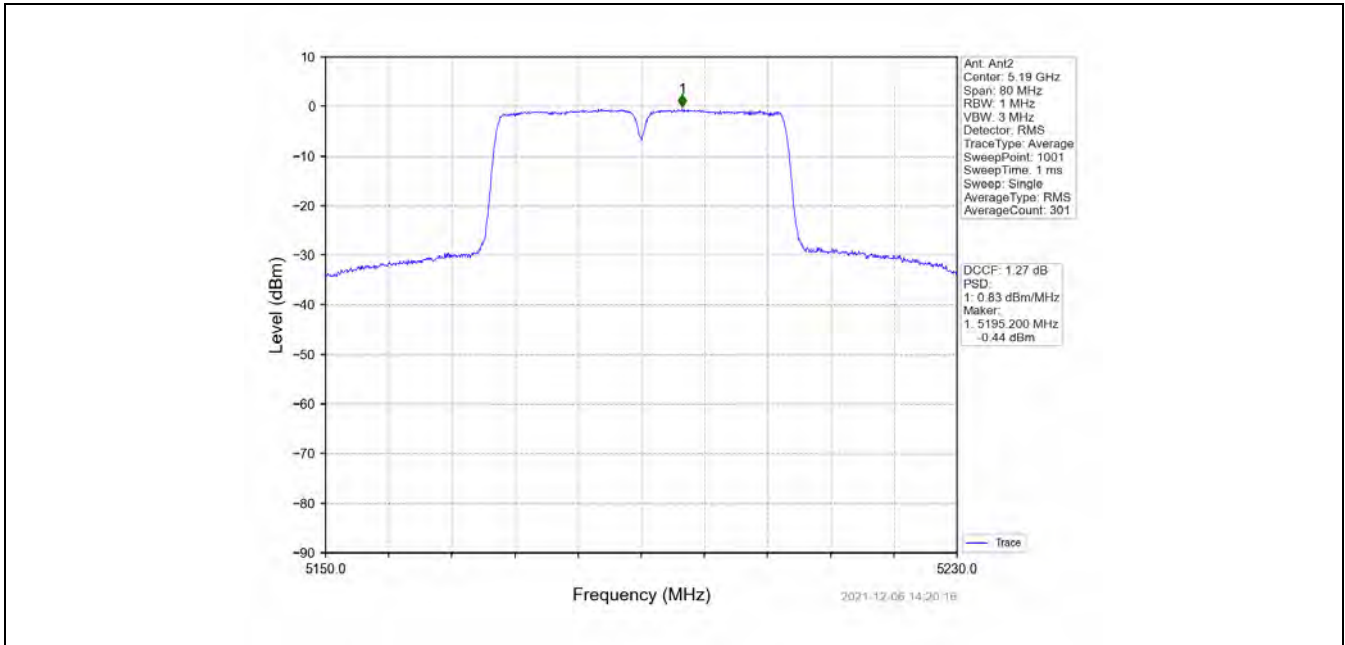
802.11n(HT40)_LCH_5190MHz_MIMO_NTNV
