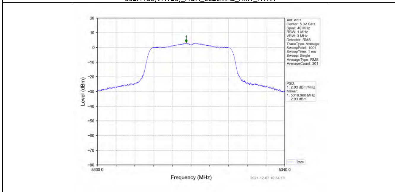
802.11ac(VHT20)_HCH_5320MHz_Ant2_NTNV
