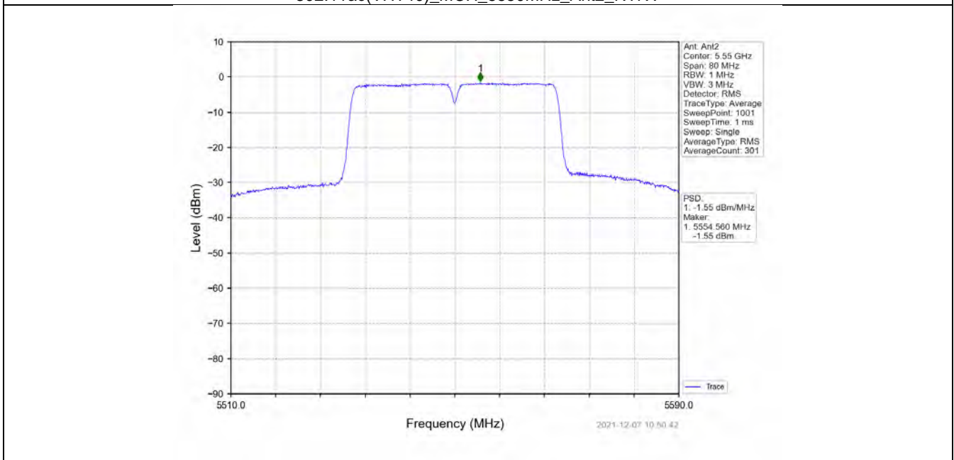
802.11ac(VHT40)_MCH_5550MHz_MIMO_NTNV
