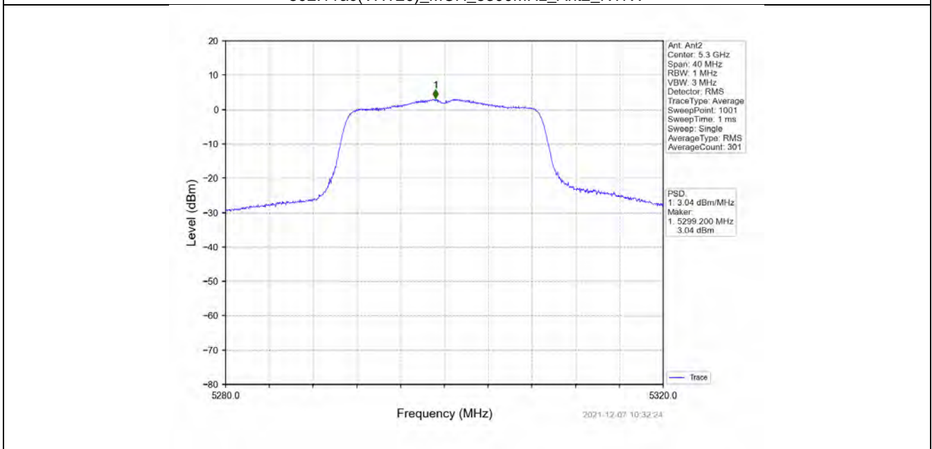
802.11ac(VHT20)_MCH_5300MHz_MIMO_NTNV
