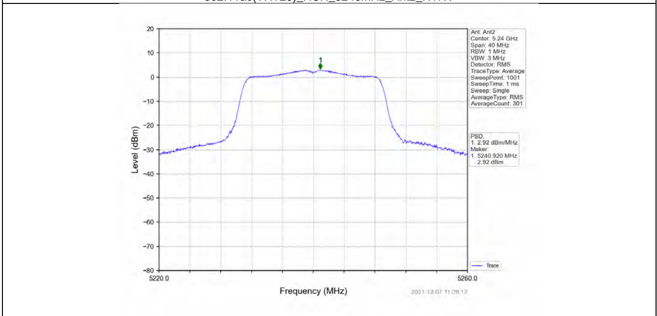
802.11ac(VHT20)_HCH_5240MHz_MIMO_NTNV
