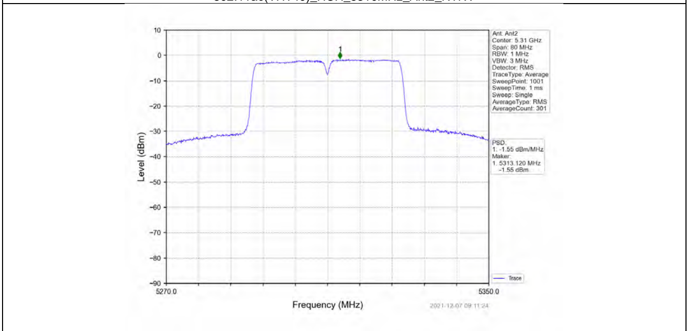
802.11ac(VHT40)_HCH_5310MHz_MIMO_NTNV
