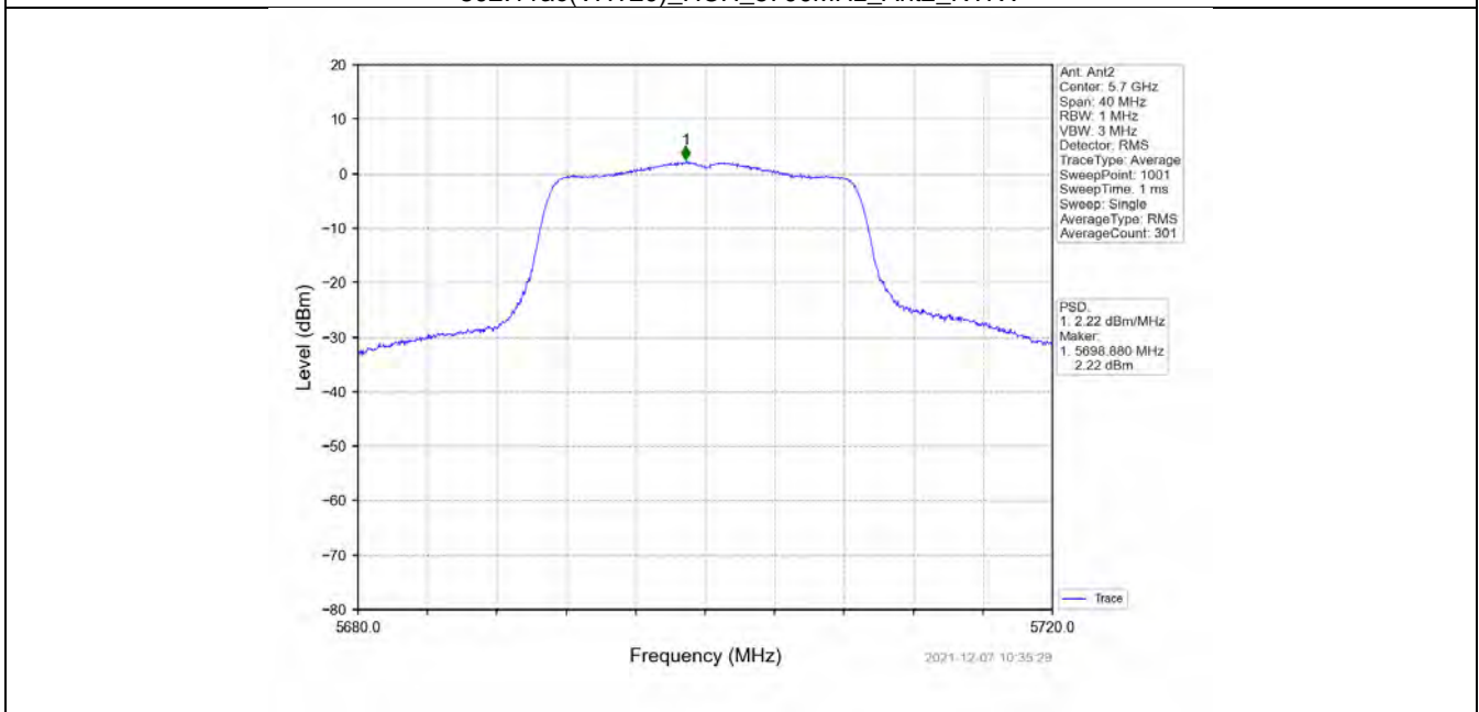
802.11ac(VHT20)_HCH_5700MHz_MIMO_NTNV
