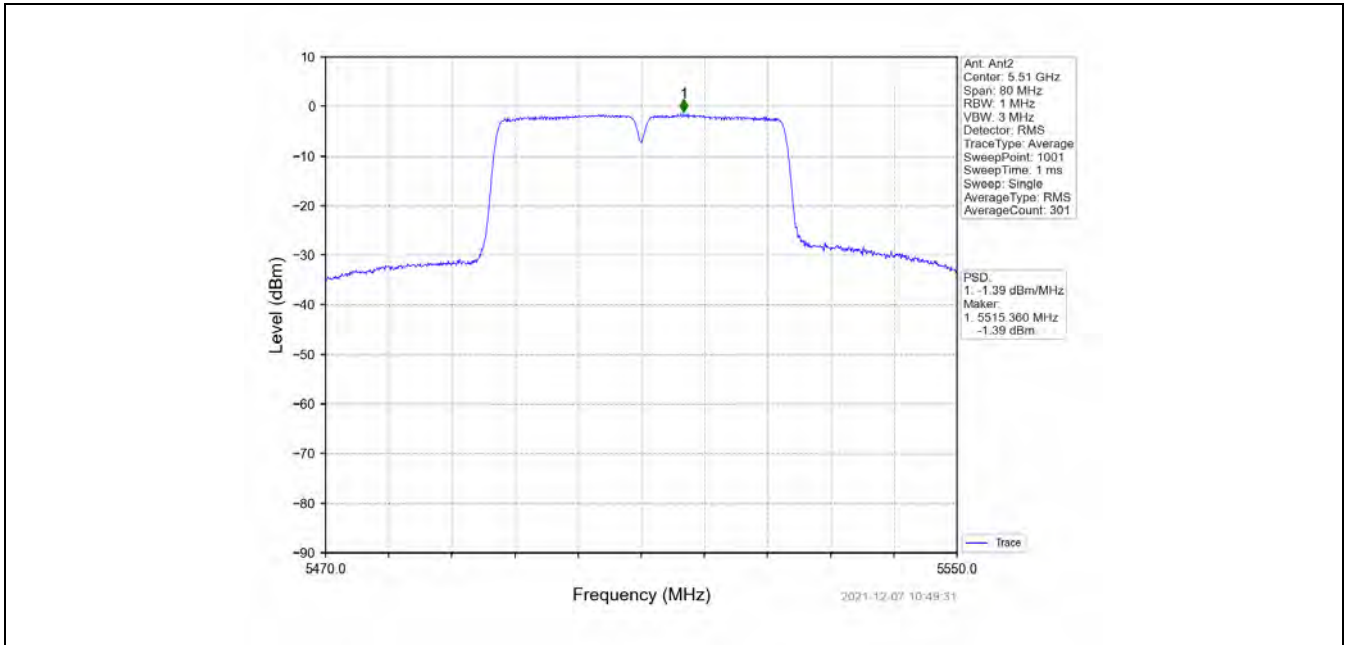
802.11ac(VHT40)_LCH_5510MHz_MIMO_NTNV
