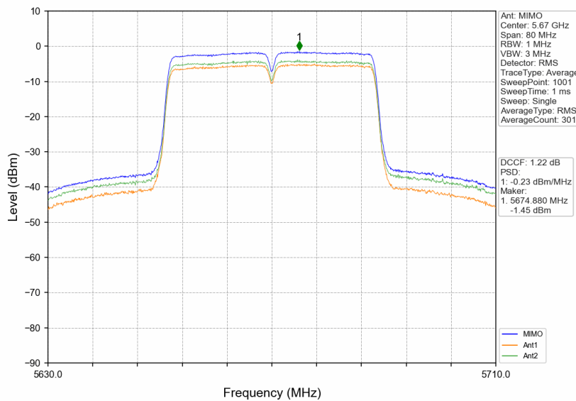
802.11ac(VHT40)_HCH_5670MHz_MIMO_NTNV
