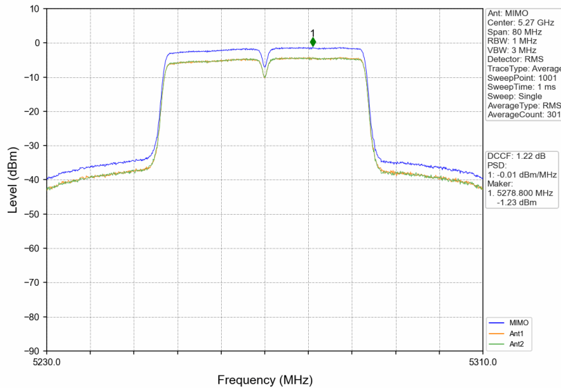
802.11ac(VHT40)_LCH_5270MHz_MIMO_NTNV
