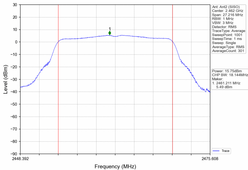
802.11g_HCH_2462MHz_Ant2 (SISO) NTVN
