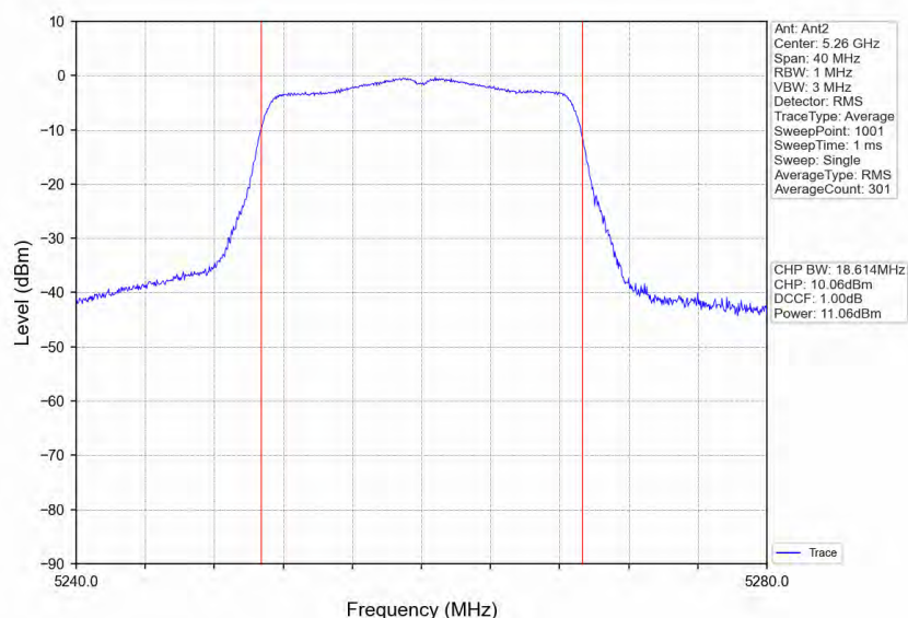
802.11ac(VHT20) LCH_5260MHz_Ant2_NTNV
