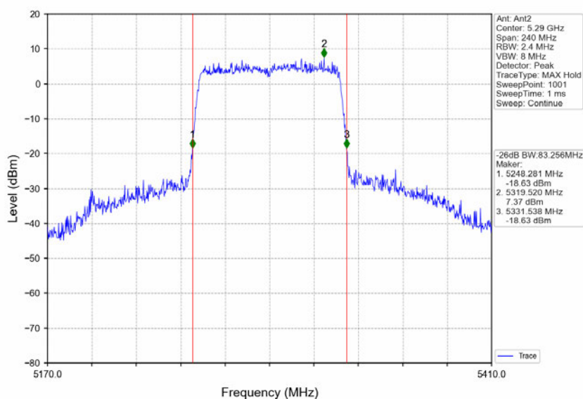
802.11ac(VHT80)_MCH_5290MHz_Ant2_NTNV
