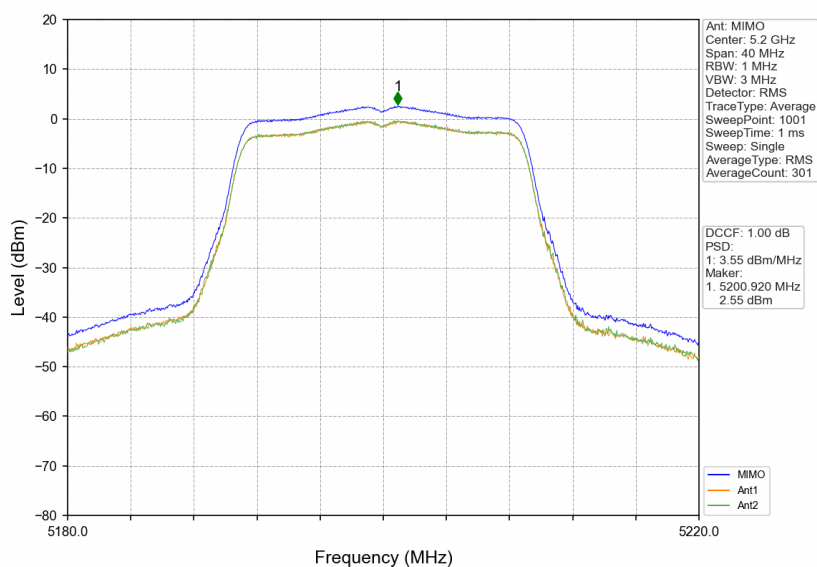
802.11ac(VHT20)_MCH_5200MHz_MIMO_NTNV
