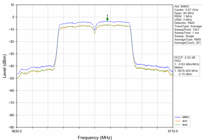
802.11n(HT40)_HCH_5670MHz_MIMO_NTNV
