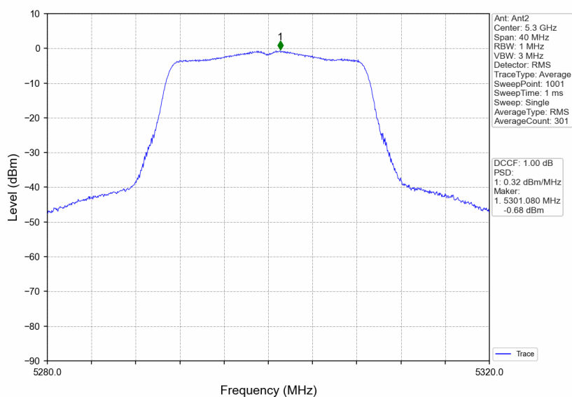
802.11ac(VHT20)_MCH_5300MHz_Ant2_NTNV
