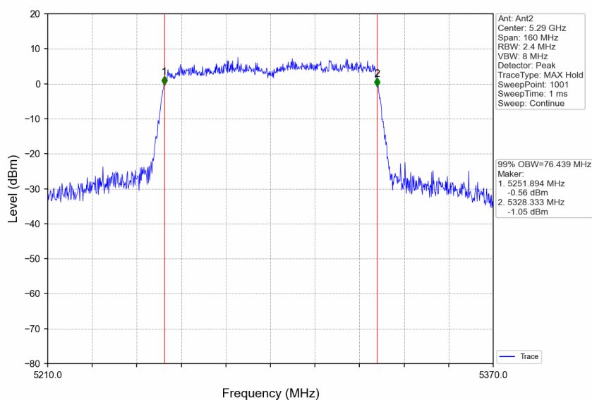
802.11ac(VHT80)_MCH_5290MHz_Ant2_NTNV
