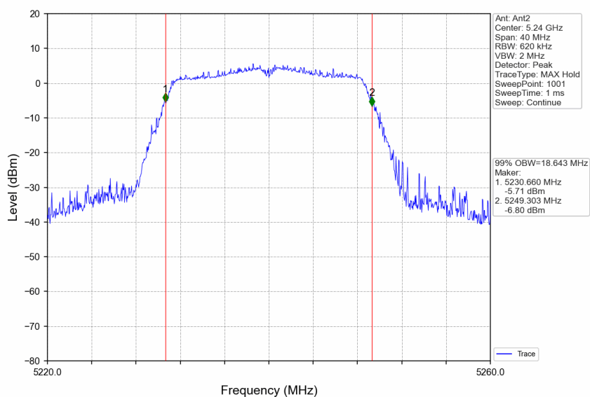
802.11ac(VHT20)_HCH_5240MHz_Ant2_NTNV
