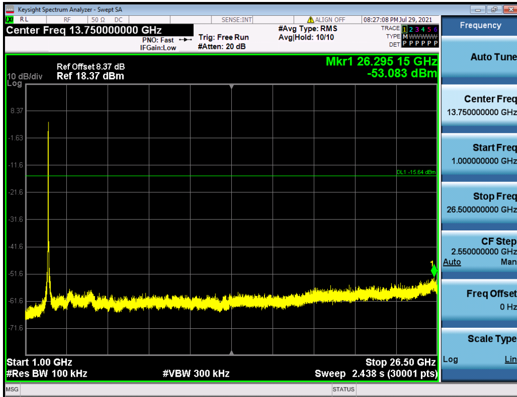
11N40SISO_Ant1_2422_1000~26500
