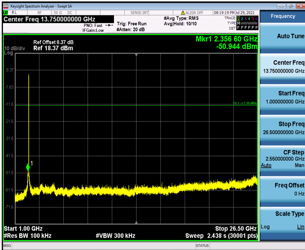
11N20SISO_Ant1_2442_1000~26500
