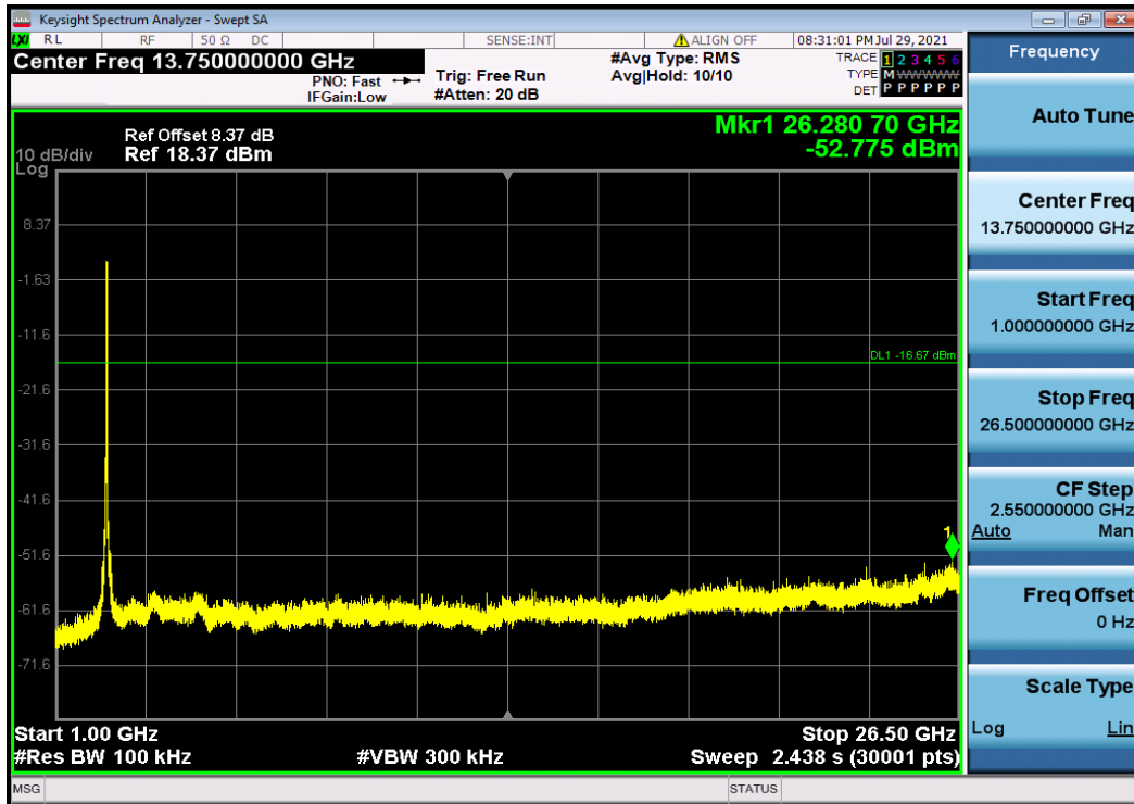
11N40SISO_Ant1_2452_0~Reference
