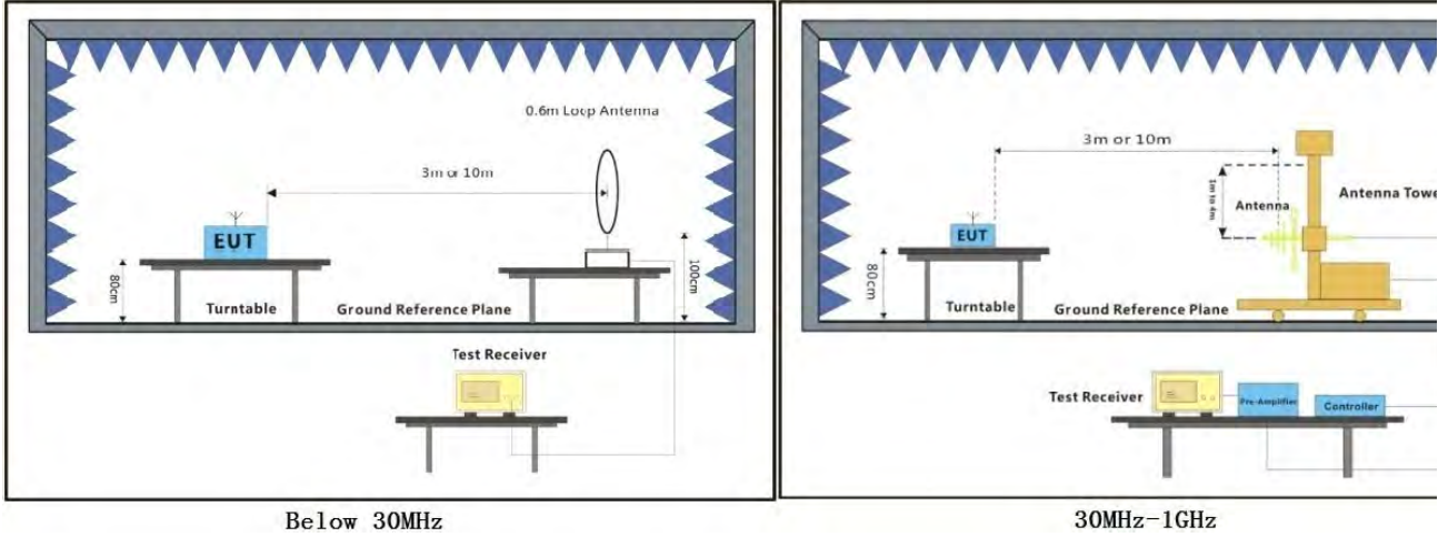
Below 30MHz
