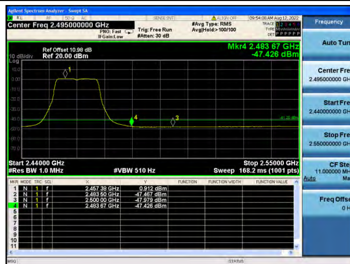
11G_Ant2_High_2462_AV
