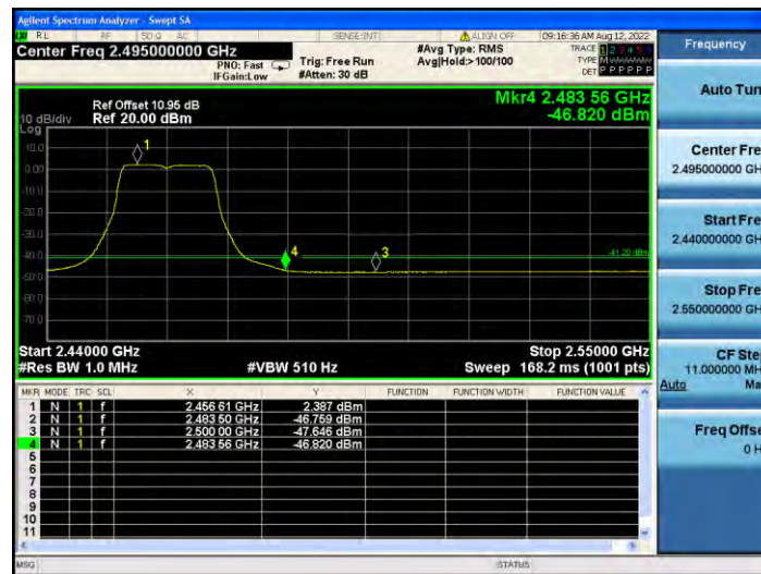
11G_Ant1_High_2462_Peak
