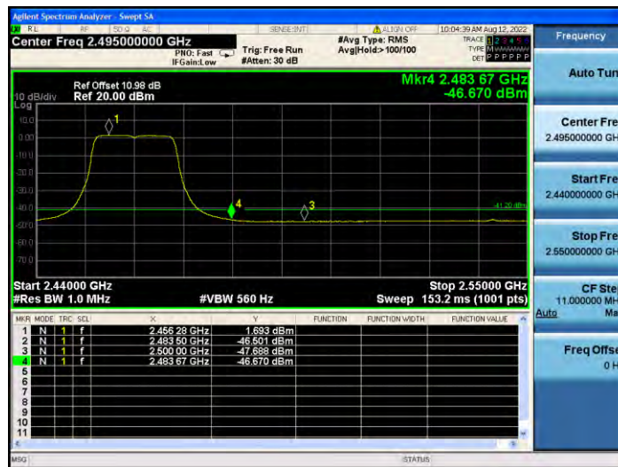
11N20MIMO_Ant2_High_2462_Peak
