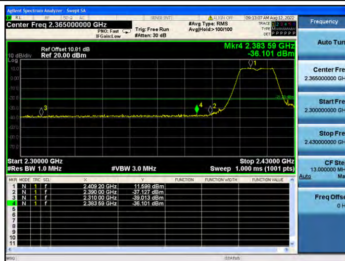
11G_Ant1_Low_2412_Peak
