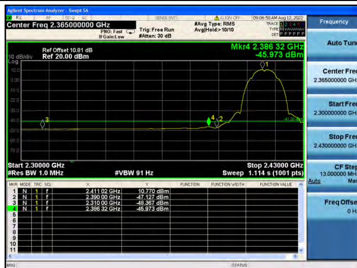
11B_Ant1_Low_2412_Peak
