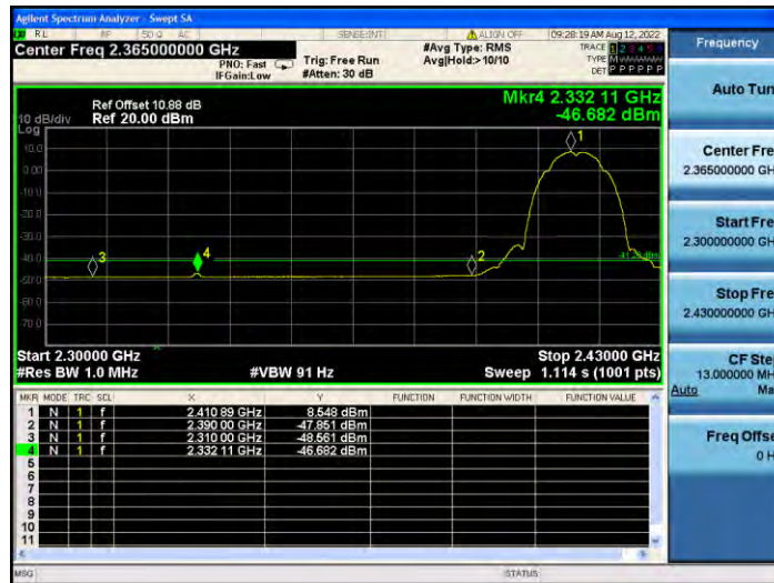
11B_Ant2_Low_2412_Peak
