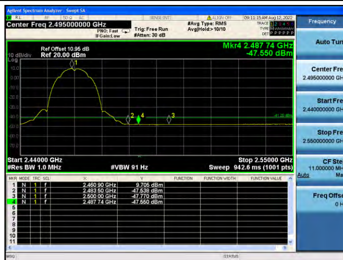
11B_Ant1_High_2462_AV
