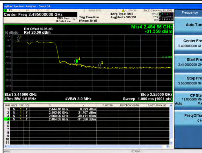
11N40MIMO_Ant1_High_2452_Peak
