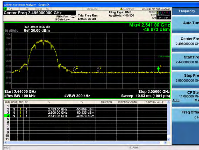
11B_Ant2_High_2462
